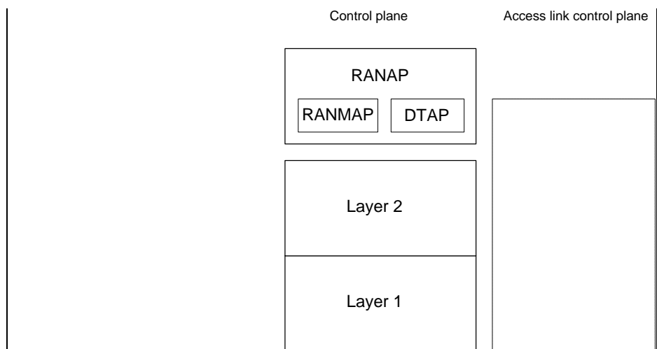
Figure 2: Transport Network Control plane protocol structure on Iub.
