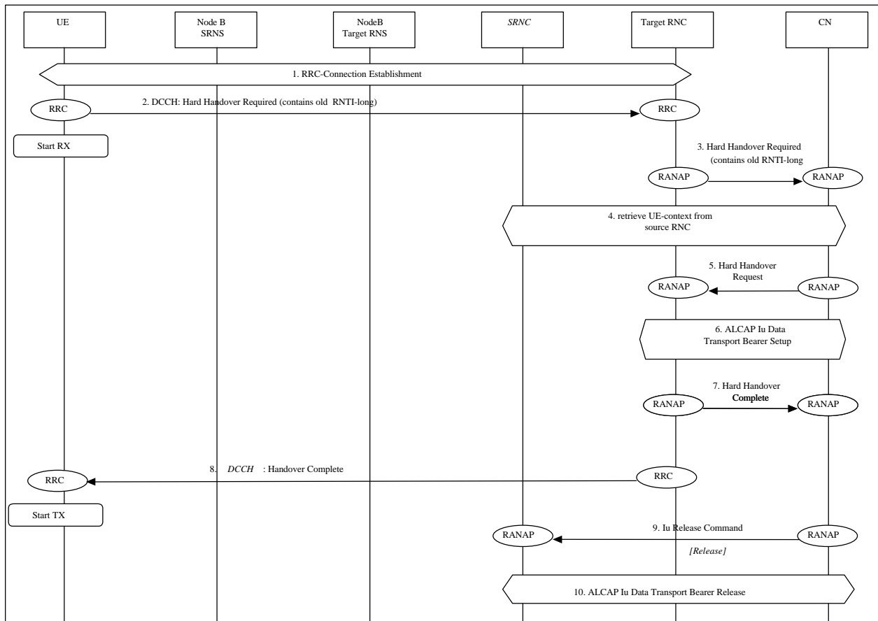
Figure 1: Inter-RNC hard handover (HO A2) for a UE in RACH/FACH state
