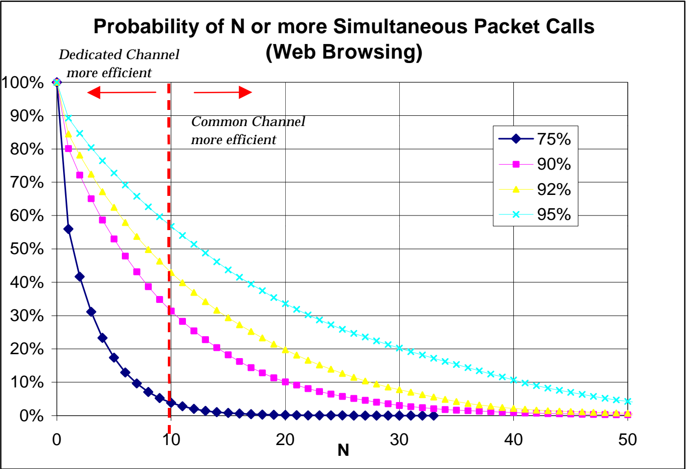
Figure 2. CDF of Number of Simultaneous Packet Calls for different Utilization Factors
