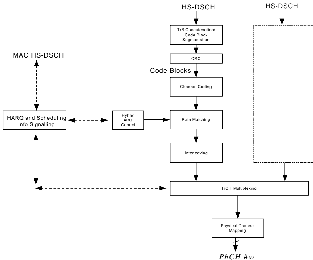
Figure 1: Proposed HSDPA Multiplex Structure [1]
