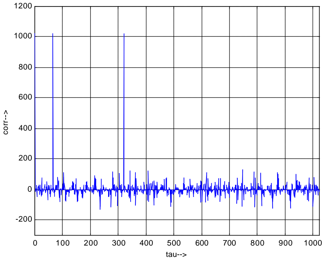
Output of cyclic correlator for \phi_g(n)
