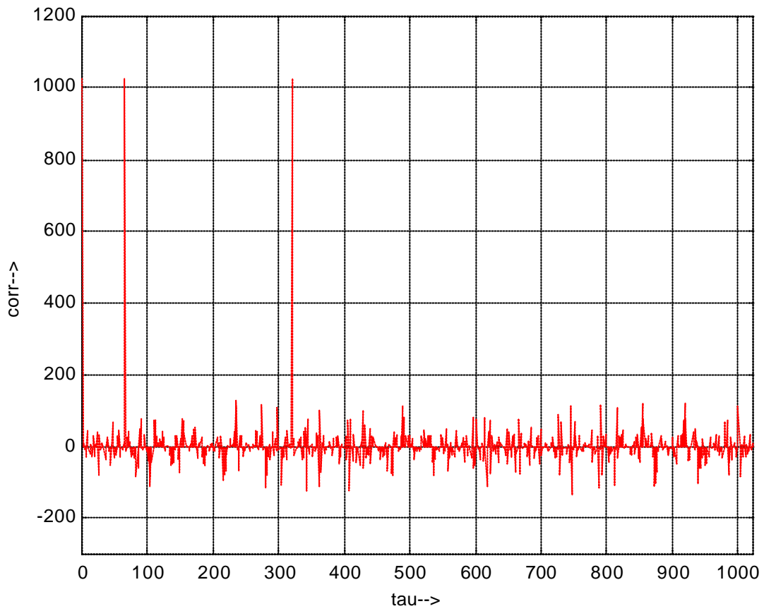
Figure 6: Cyclic correlator output for correlation with s'(n)
