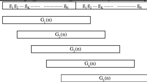
Figure 4: Deriving different code offset versions of the basic sequence g(n)
