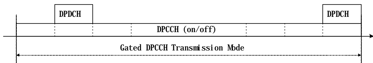
Figure 3. DPDCH Transmission during gated DPCCH transmission mode
