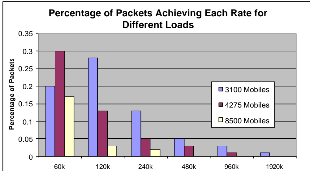
Figure 6. Percentage of Packets as function of throughput for the different loading levels. Mean distance from serving site for each throughput level, measured per packet The rate of each packet is calculated as in the previous section. A sample output graph is shown in the Figure 7.
