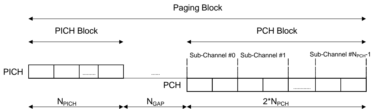
Figure 2019: Paging Sub-Channels and Association of PICH and PCH blocks
