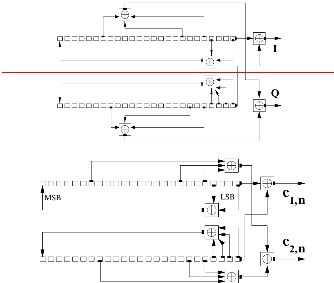
Figure 4. Configuration of uplink scrambling code generator
