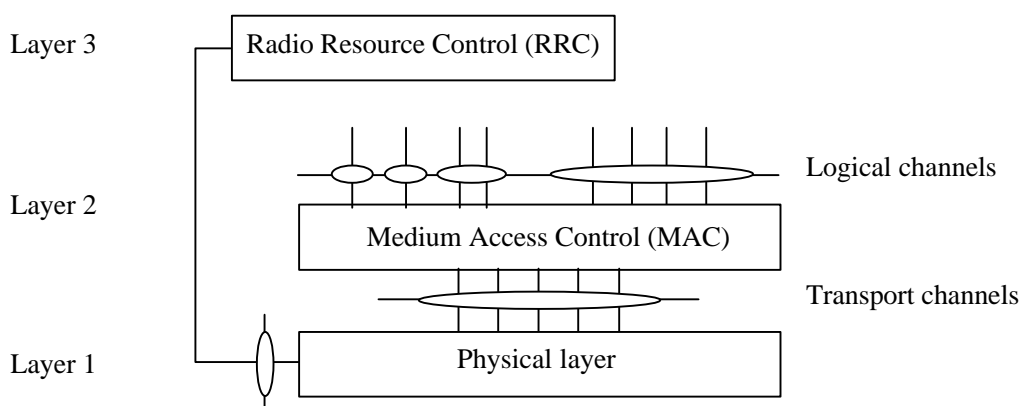
Fig. 54-1 Radio interface protocol architecture around the physical layer
