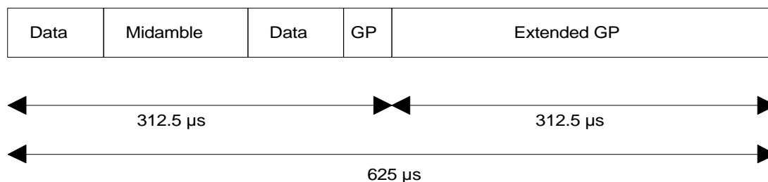
Figure 4 Access burst 1, GP denotes the guard period
