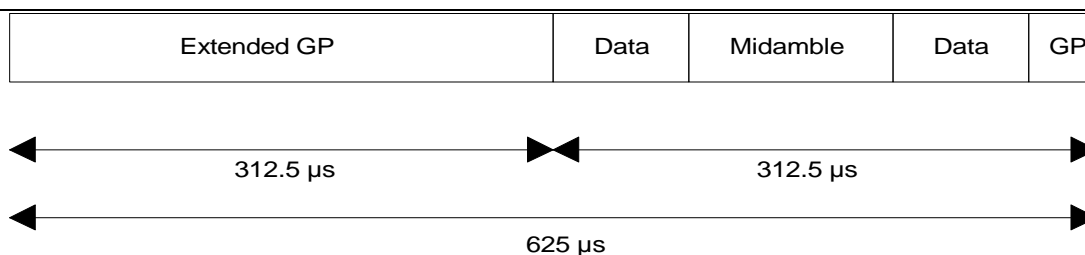
Figure 5 Access burst 2, GP denotes the guard period
