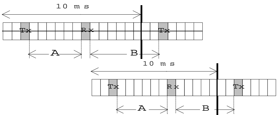
Figure: Possible idle periods in a 16-TS frame with two occupied timeslots-TS .
