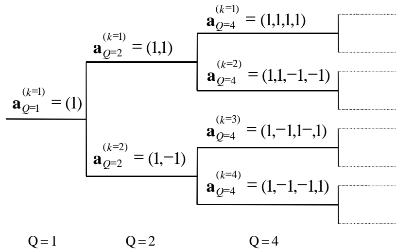
Figure 2: Code-tree for generation of Orthogonal Variable Spreading Factor (OVSF) codes.
