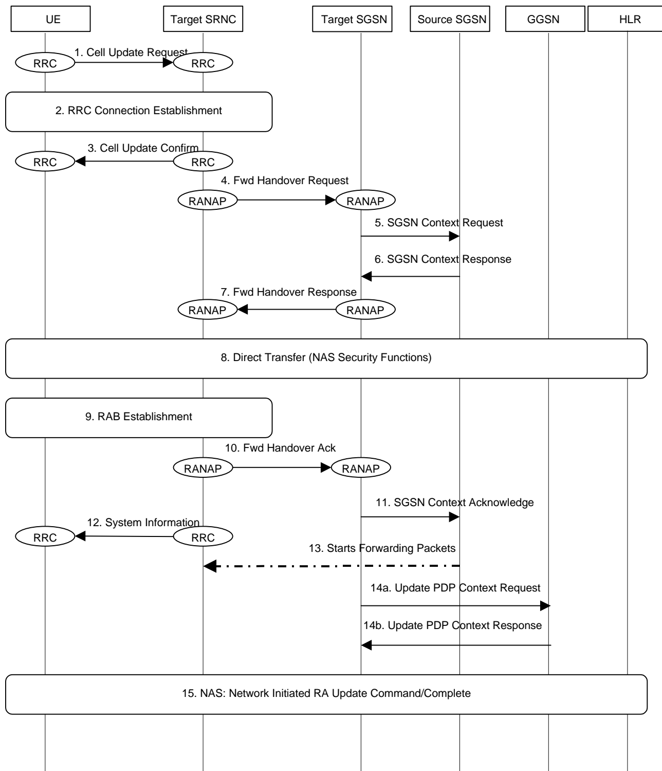
Figure 3: GPRS to UMTS cell reselection (Cell Update)
