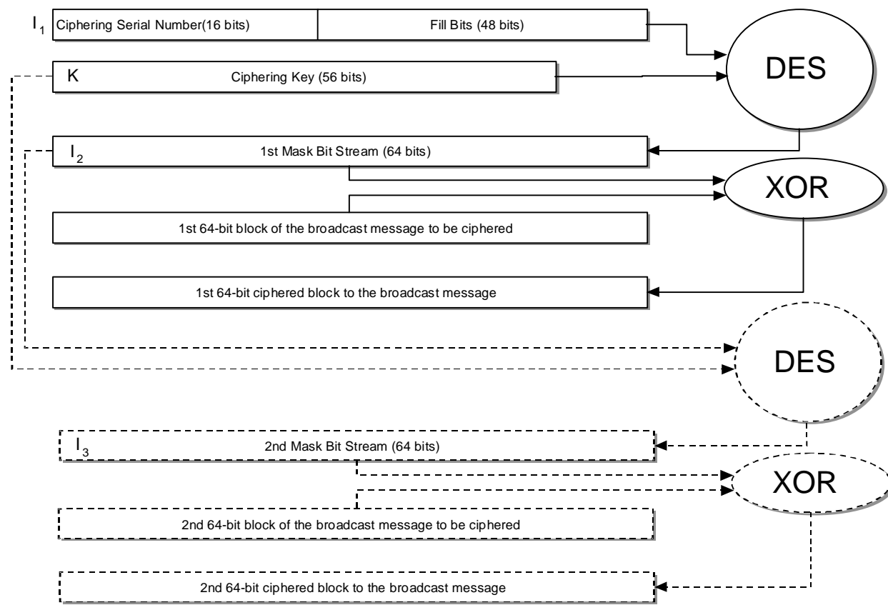
Figure 7.4: Data Assistance Ciphering Algorithm
