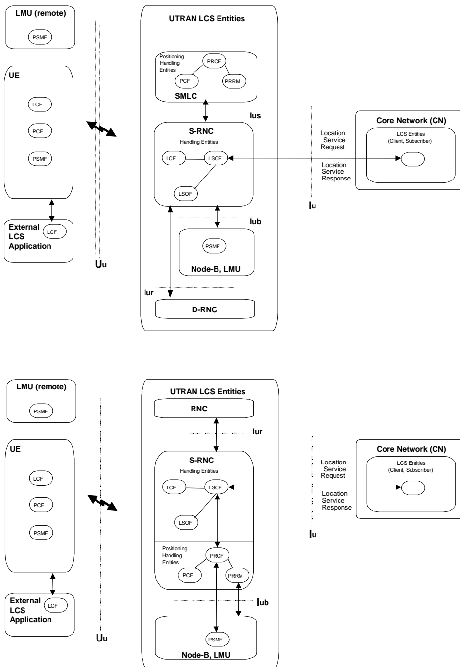
Figure B.1: UTRAN UP Functional Entities
