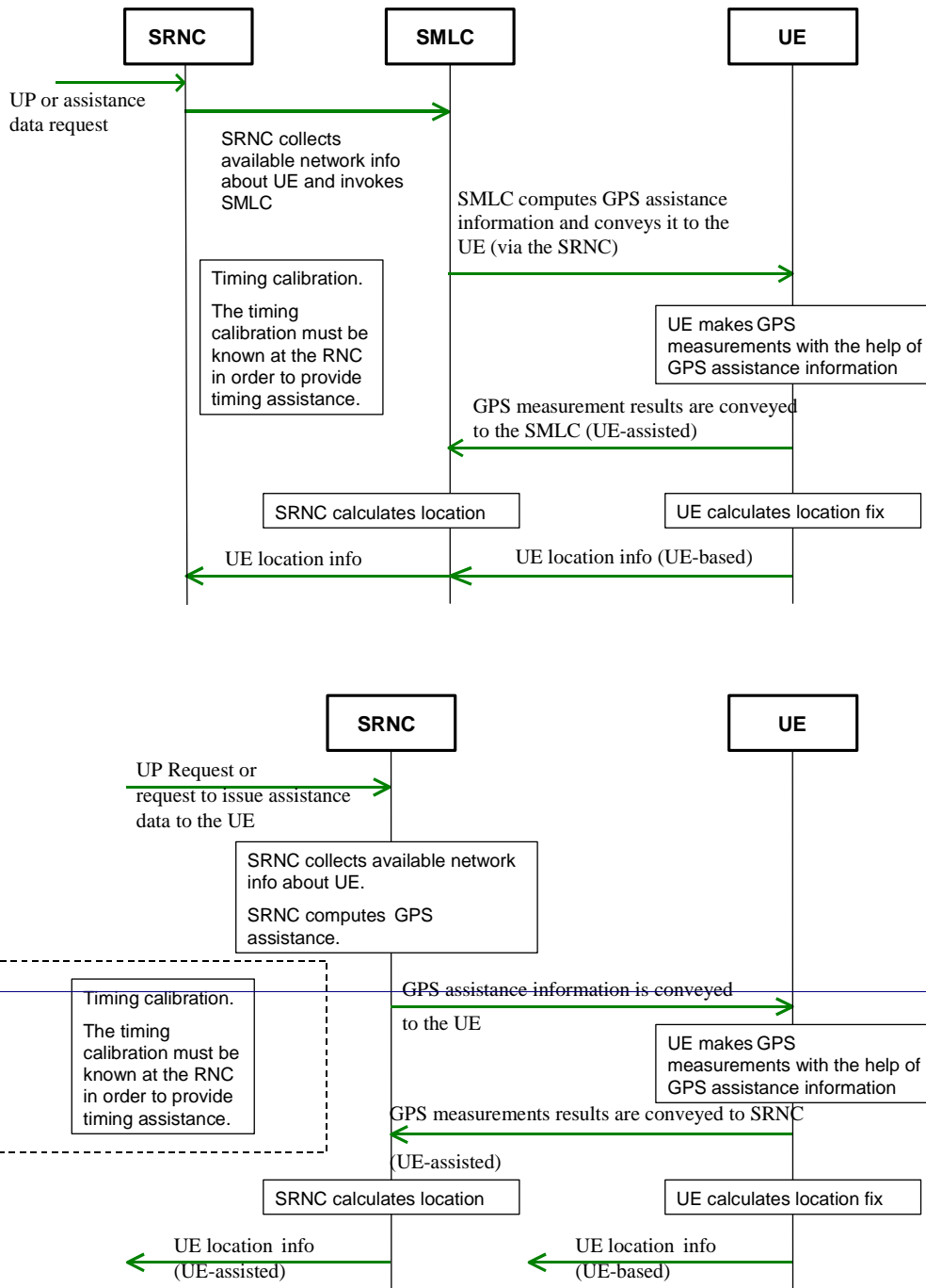
Figure 10.1: Network-assisted GPS methods
