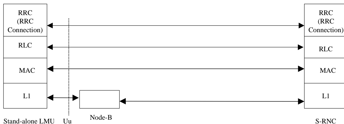
Figure 7.5: Signalling between an RNC and a Stand-Alone LMU using a signalling bearer
