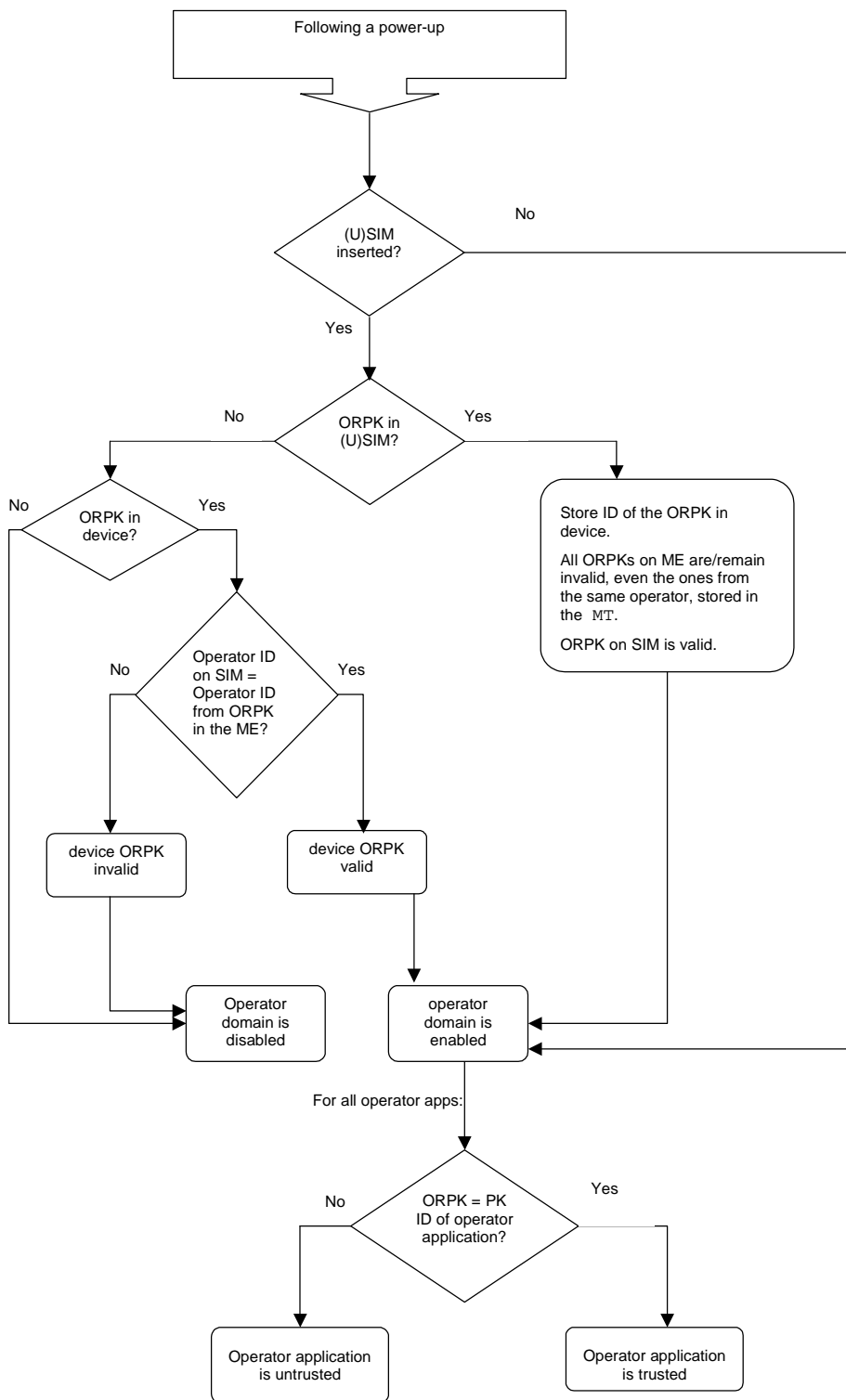
Figure 9: MExE device behaviour on power up
