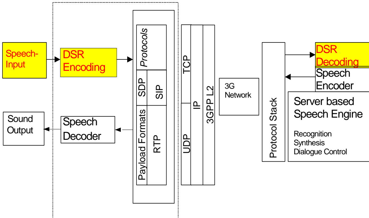
Figure 1: DSR Architecture
