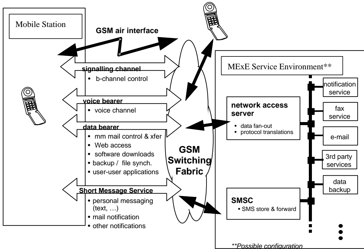
Figure 1: Generic MExE architecture
