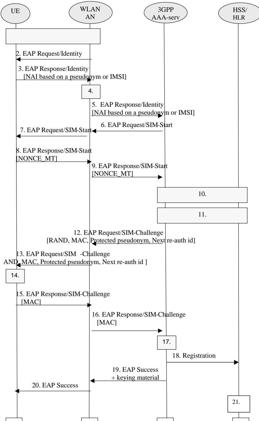
Figure 5: Authentication based on EAP SIM scheme
