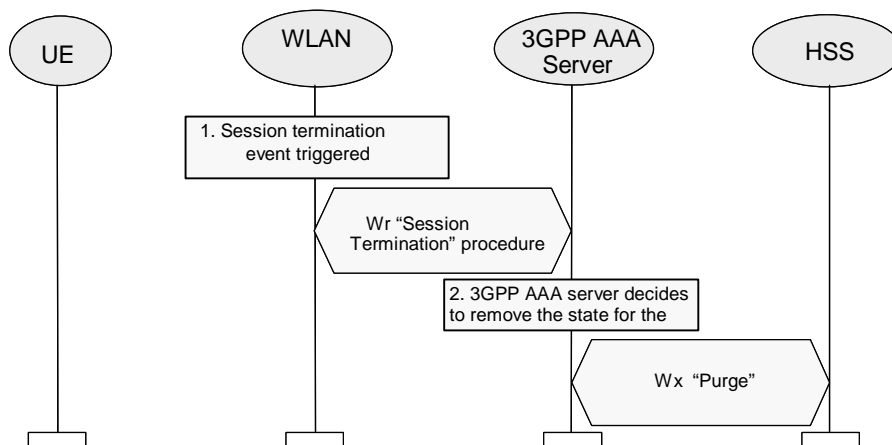
Figure 7.6: WLAN initiated disconnection procedure
