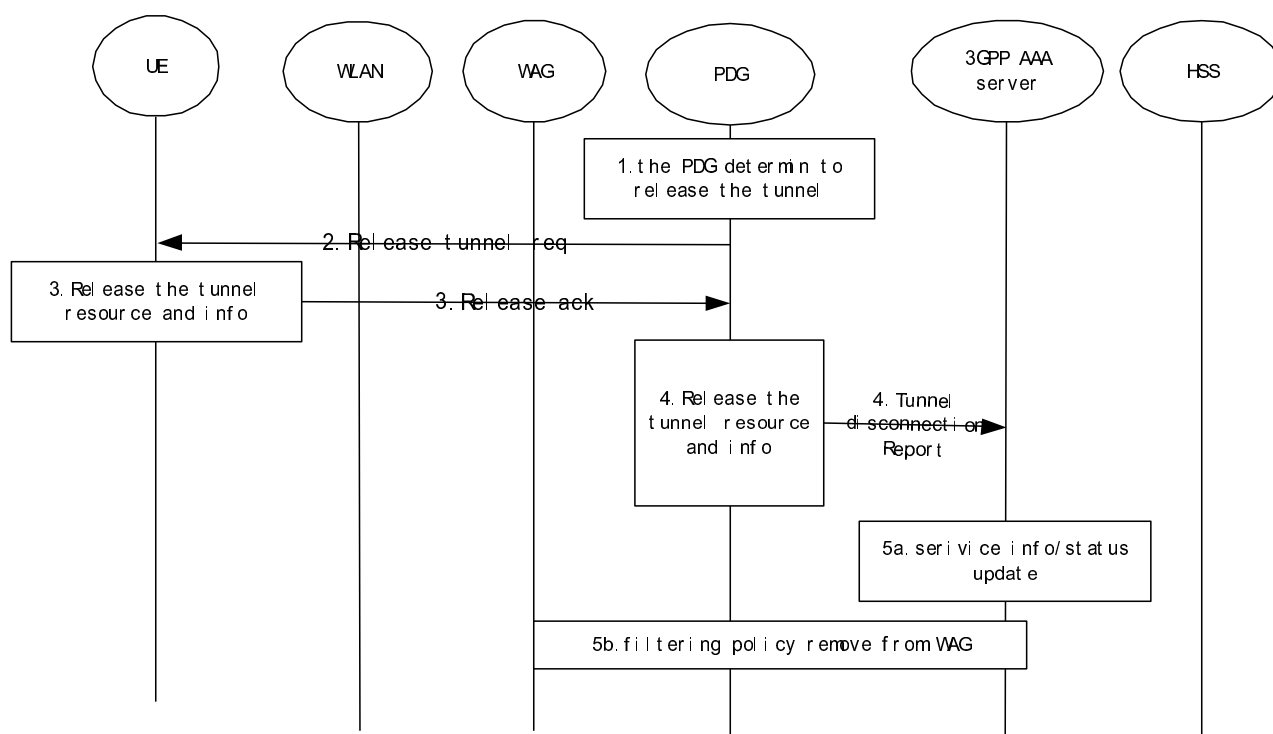
Figure 7.13: The network initiated tunnel disconnection
