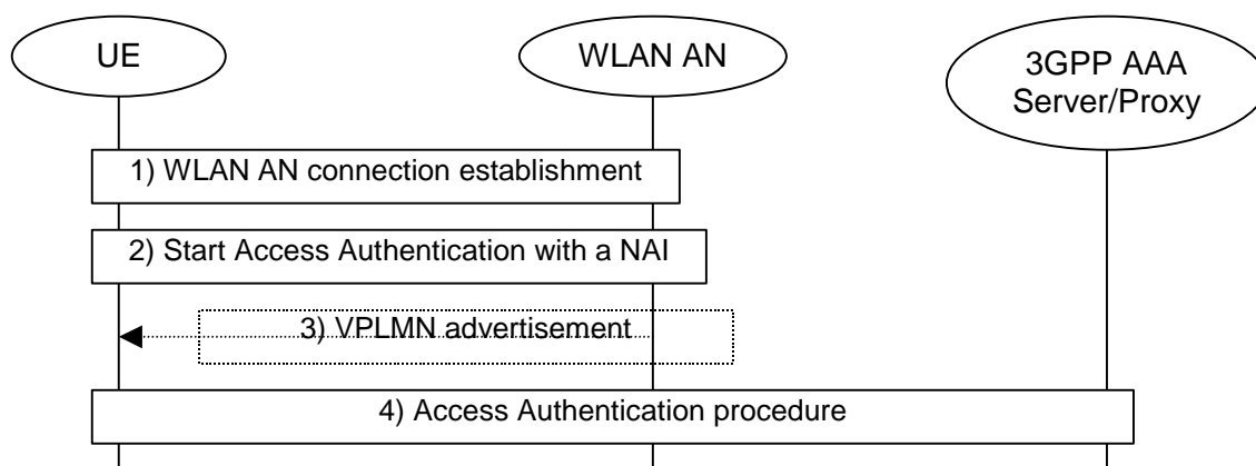
Figure 7.1: I-WLAN and VPLMN selection procedure
