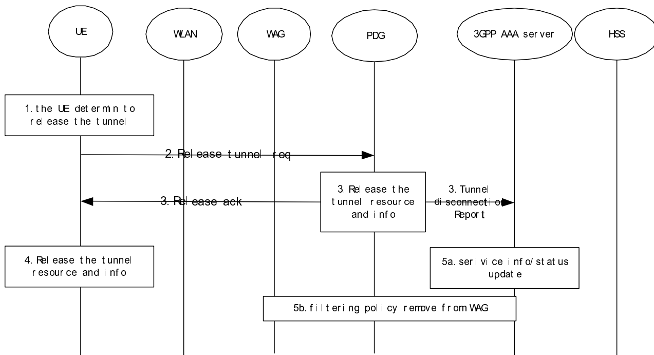
Figure 7.12: WLAN UE initiated tunnel disconnection
