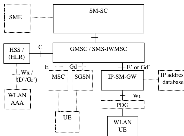
Figure D.1: Architecture for SMS interworking with IP attached terminal
