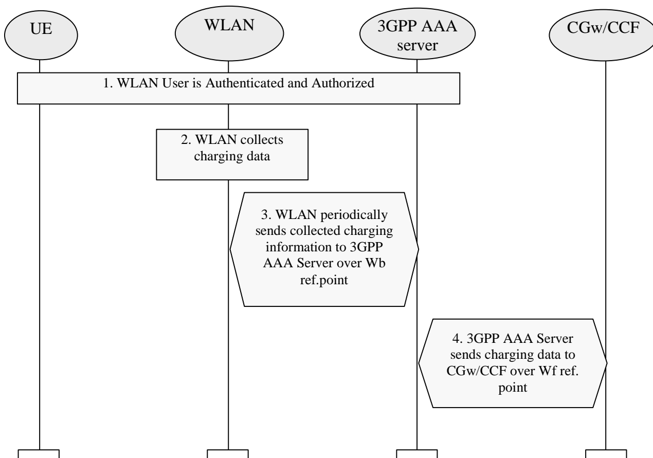
Figure 7.8: Charging Procedure for Offline Charged Subscribers
