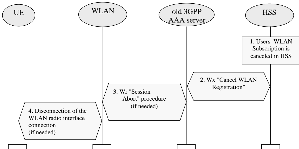
Figure 7.5: Cancellation of WLAN Registration Procedure
