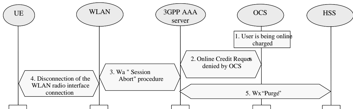
Figure 7.7: OCS Initiated Disconnection Procedure
