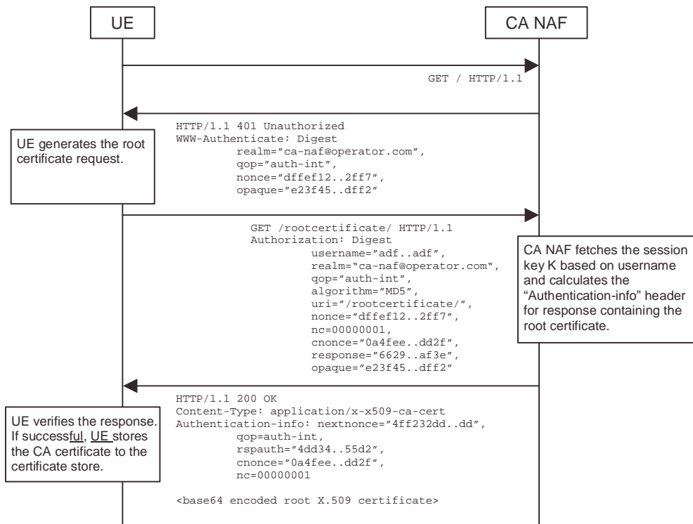
Figure 5: CA certificate delivery with HTTP Digest authentication.
