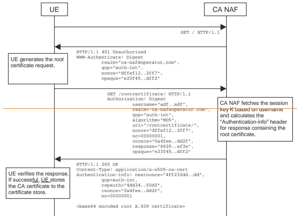
Figure 5: CA certificate delivery with HTTP Digest authentication.
