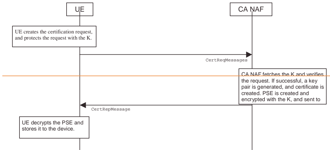
Figure 4: Certificate request using centralized scheme of CMP.
