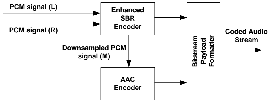
Figure 2 Parametric stereo AAC block diagram
