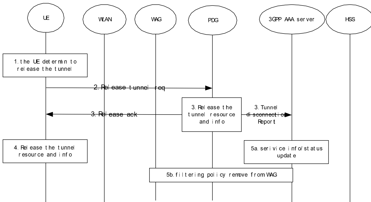
Figure 7.10 WLAN UE initiated tunnel disconnection
