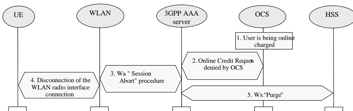
Figure 7.5 OCS Initiated Disconnection Procedure
