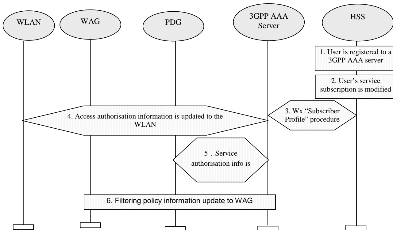
Figure 7.3 Authorization information Update Procedure
