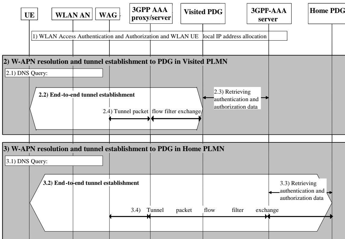
Figure 7.8. Example message flow to WLAN UE-Initiated tunnel establishment
