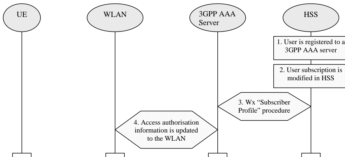
Figure 7.2 Subscriber Profile and access authorization info Update Procedure
