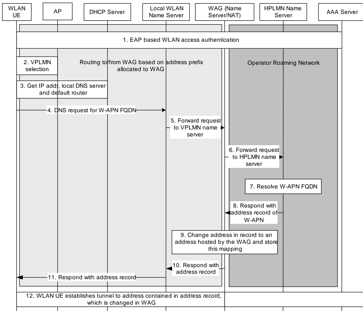
Figure C.2.1: DNS controlled reverse NAT procedure
