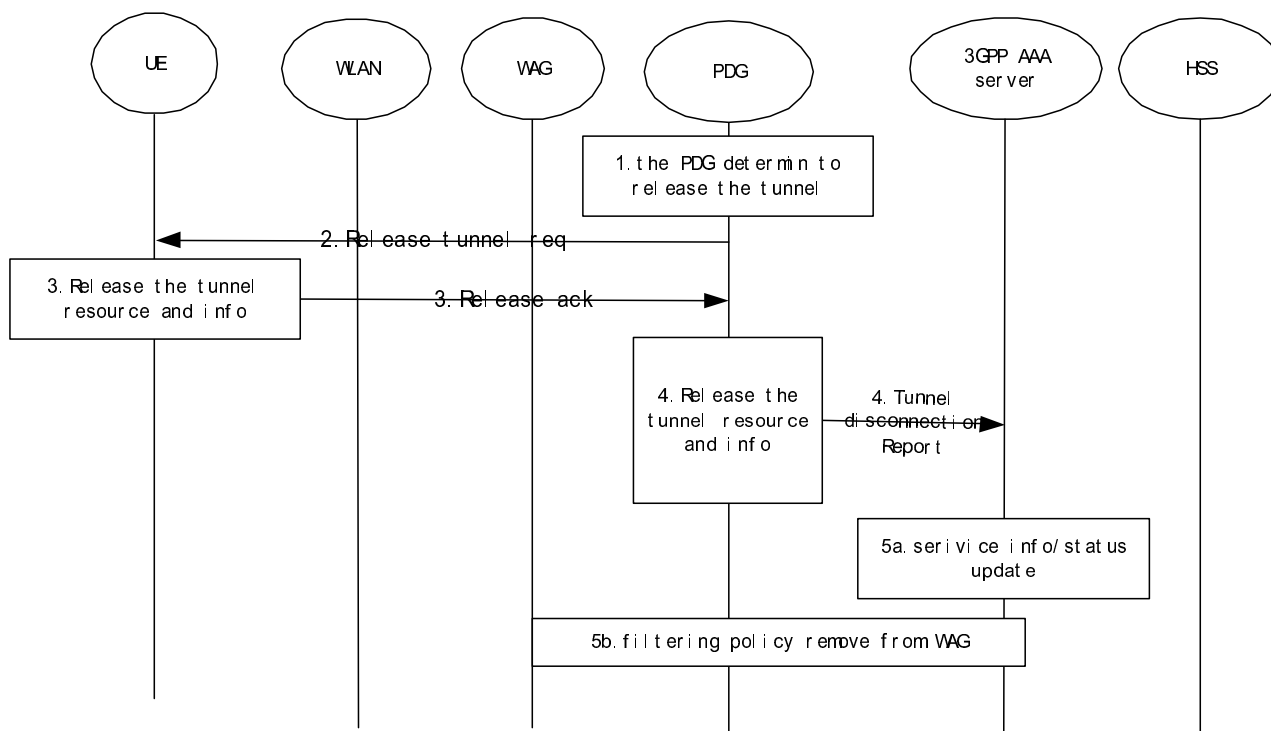
Figure 7.11 the network initiated tunnel disconnection
