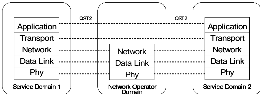
Figure 9 – Interactions between Service Domains via a Network Operator Domain
