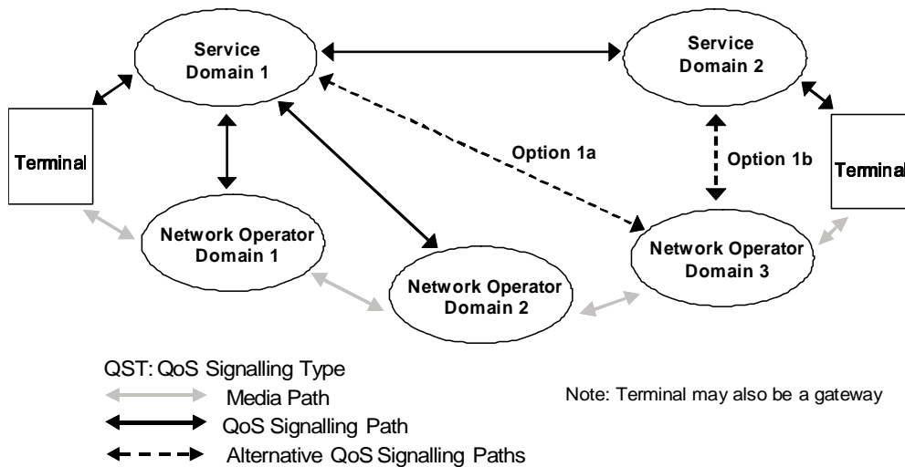
Figure 5 - Call involving Multiple Network Operator and Service Domains (Option 1)
