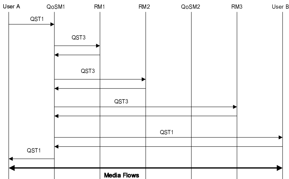
Figure 13 –QoS Signalling Option 1a
