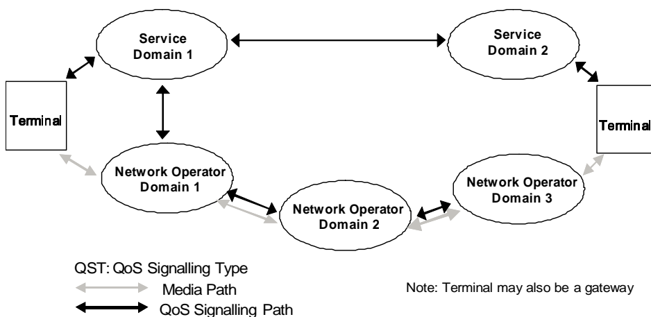
Figure 6 - Call involving multiple Network Operator and Service Domains (Option 2)
