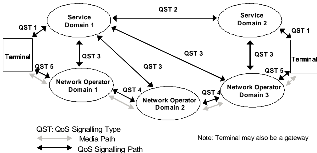
Figure 7 – QoS Signalling Types for Calls Involving Multiple Network Operator and Service Domains
