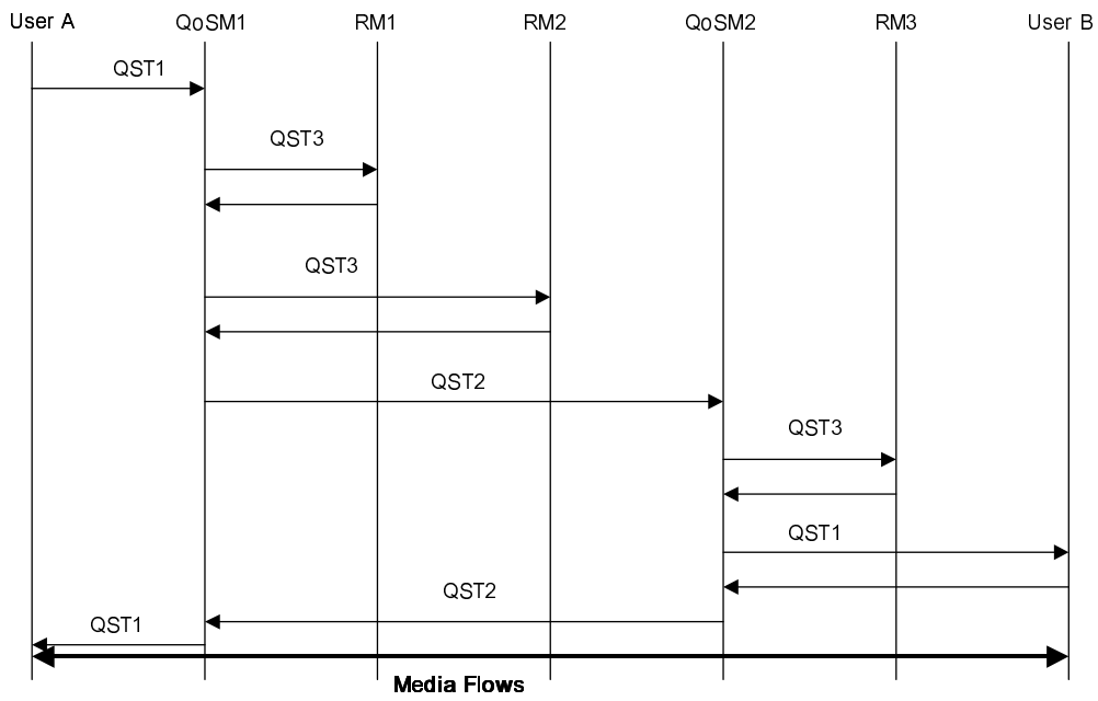
Figure 14 –QoS Signalling Option 1b
