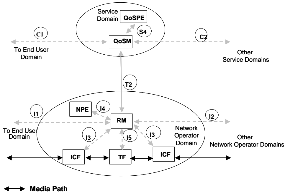
Figure 4 - Relationship between QoS Functional Entities
