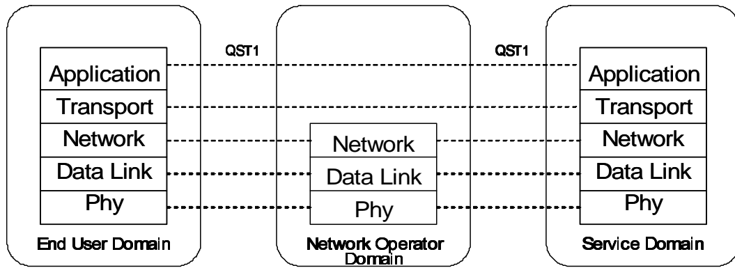
Figure 8 – Interactions between an End User Domain and a Service Domain via a Network Operator Domain
