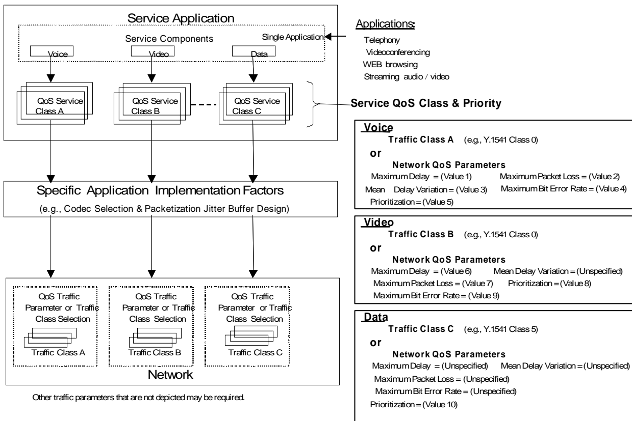
Figure 2 - QoS Classification at Service, Application, and Network Levels
