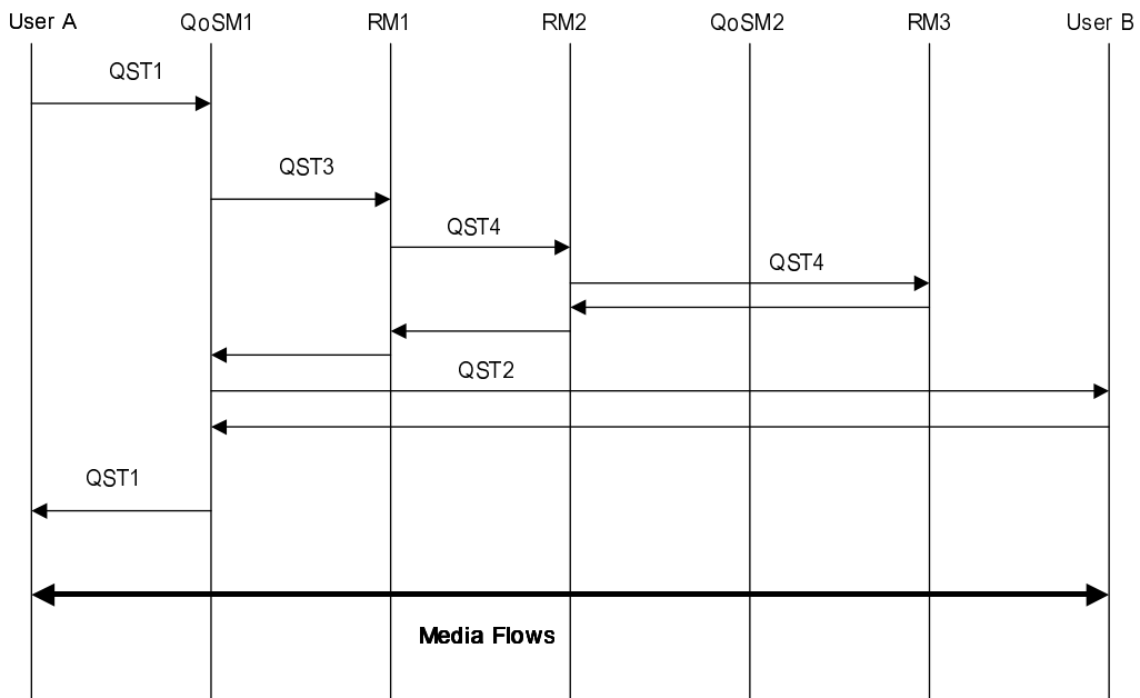
Figure 15 – QoS Signalling Option 2
