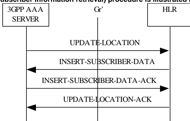
Figure X.1. gprsLocationUpdate procedure
