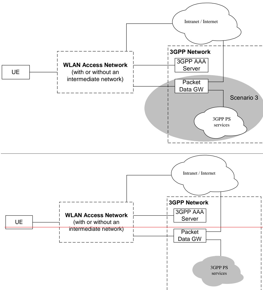
Figure 4.1: Simplified WLAN Network Model. The shaded area refers to scenario 3 functionality
