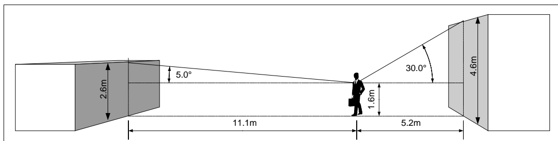
Figure 4.3.5-2: Masking Angle Concept
