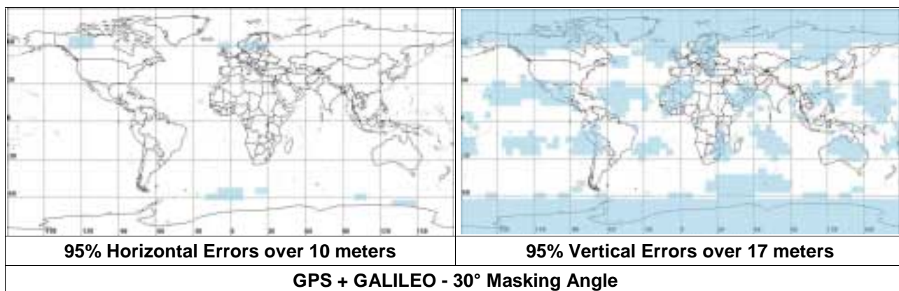
Figure 4.3.5-4: GPS + GALILEO - 30° Masking Angle
