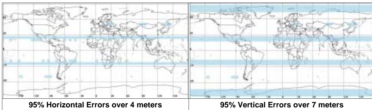
Figure 4.3.4-1: GALILEO Single Frequency - 5° Masking Angle
