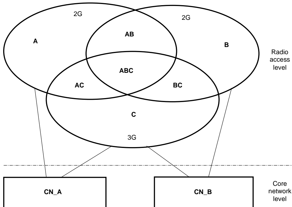
Figure B.1: Basic Network Sharing Architecture
