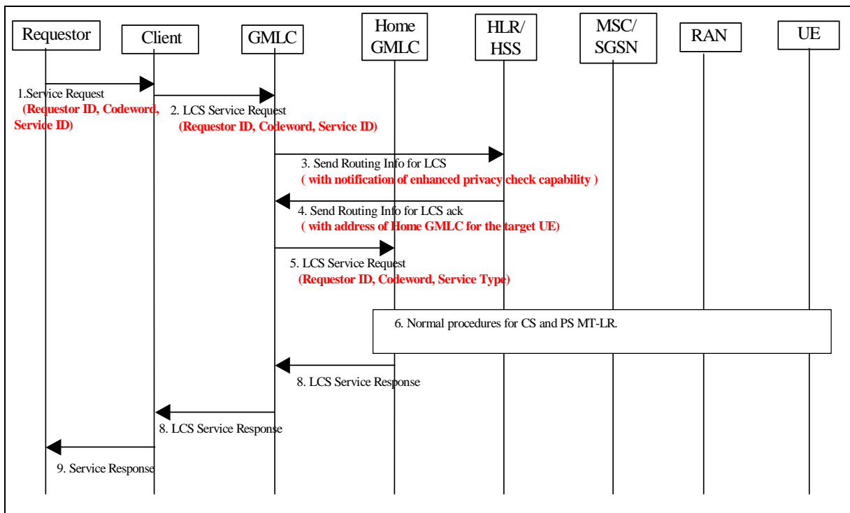
re 7.3.2; General information flow for the architectural alternative with the Home GMLC
