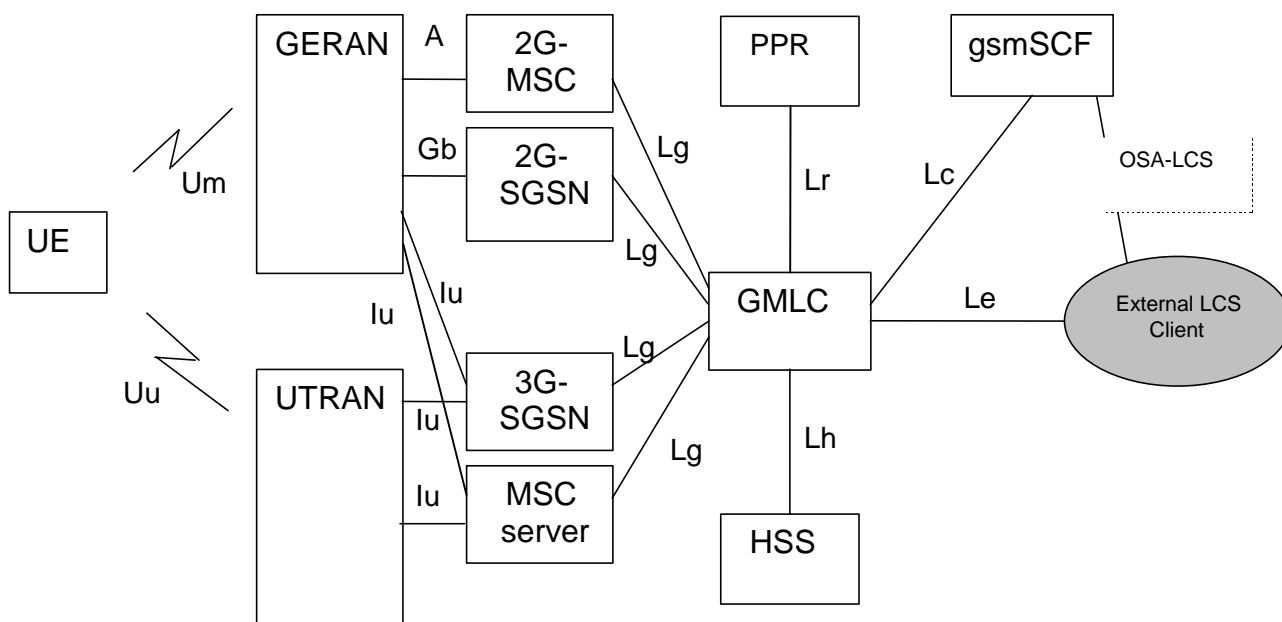
Figure 7.1.1; LCS architecture alternative with PPR attached to GMLC
