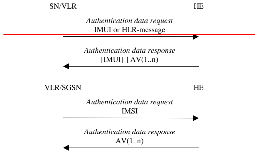
Figure 6: Distribution of authentication data from HE to VLR/SGSN
