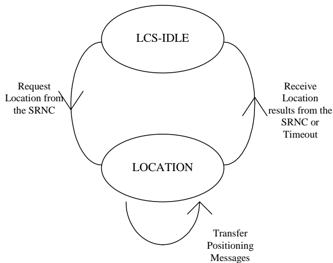
Figure 8.2; State Transitions in the 3G-VMSC
