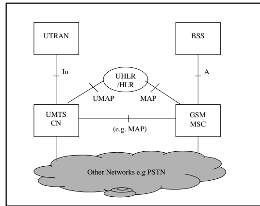
Figure xx. Inter-Operability between GSM and UMTS
