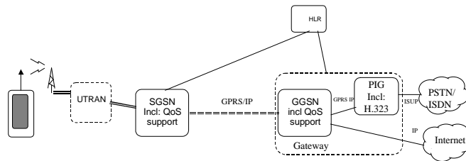
Figure 41: Evolved GPRS/IP support for Multi-media services
