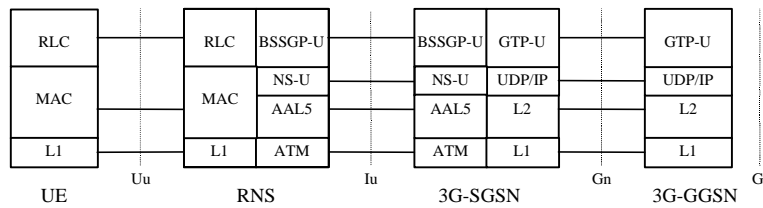
Figure 33: User Plane Protocol Architecture for Proposal 1
