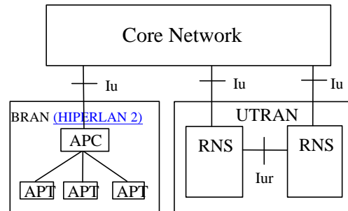
Figure 25: HIPERLAN 2 UMTS interworking.
