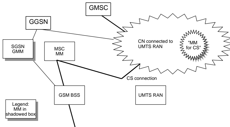
Figure 39 After HO from UMTS to GSM.
