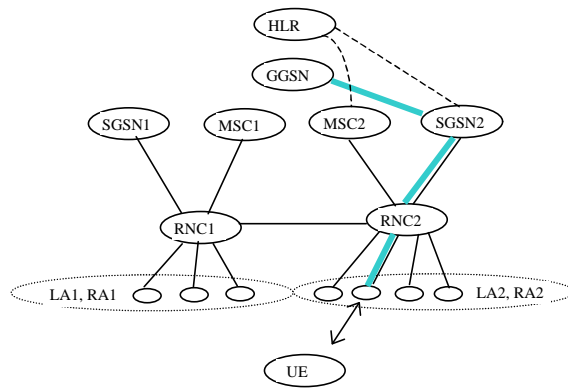
Figure 18 After the SRNS relocation and location registration
