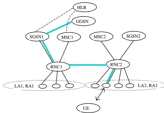
Figure 17 Before the SRNS relocation and location registration
