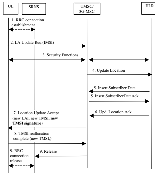
Figure 8: Attach Procedure using TMSI signature
