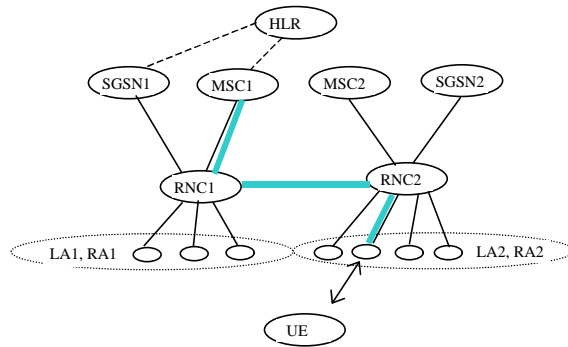
Figure 14 Before the SRNS relocation and location registration
