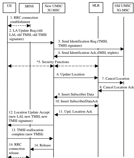
Figure 9: Location Update using TMSI signature
