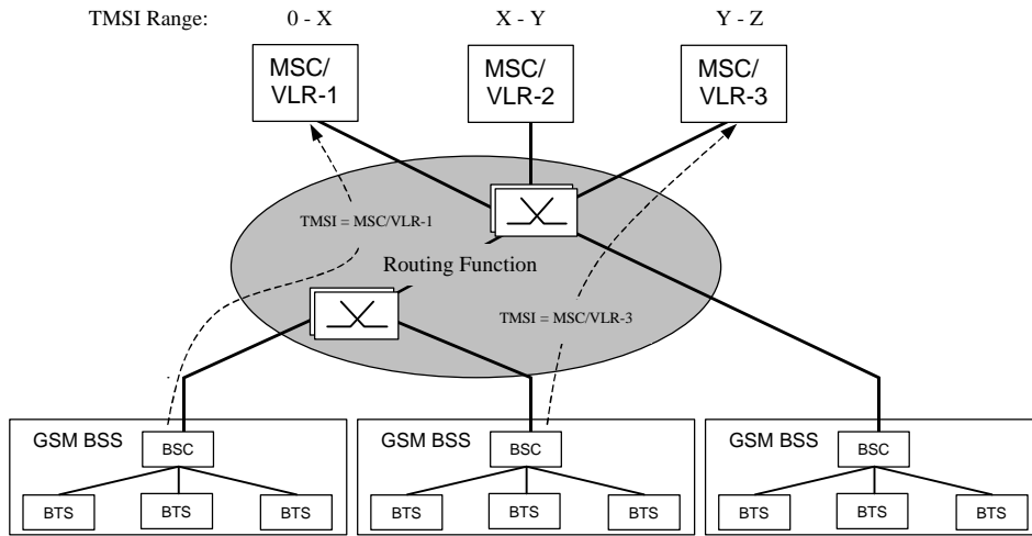
Figure 42: Example of GSM Turbo-Charger Network Architecture
