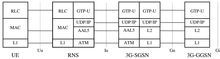
Figure 34: User Plane Protocol Architecture for Proposal 2
