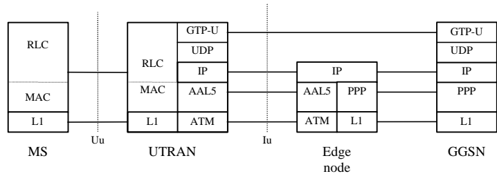
Figure 35: User Plane Protocol Architecture for Proposal 3
