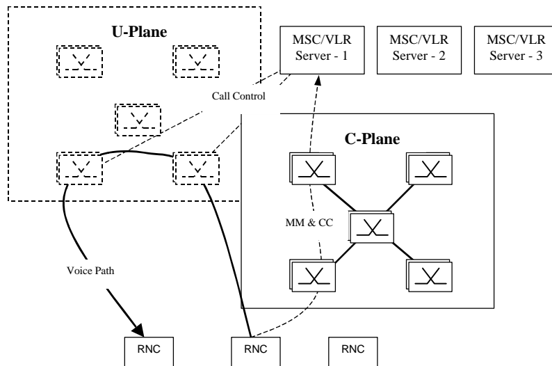
Figure 43: Example of UMTS Turbo-Charger Network Architecture
