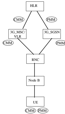
Figure 22 Split MM Instances for Separate Nodes
