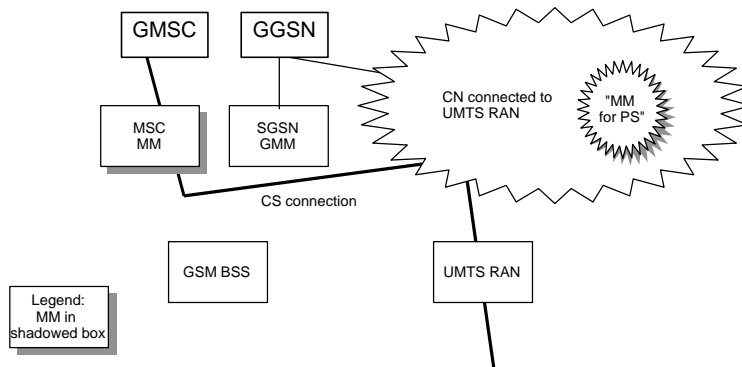
Figure 37 After HO to UMTS from GSM.
