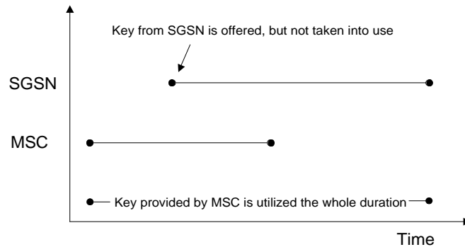
Figure 28. One ciphering key use in the UTRAN
