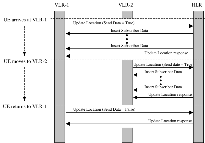
Figure 27: Example message flow in a Super-Charged network.
