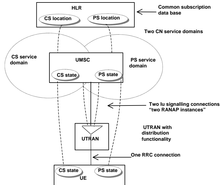
Figure 2: Overview of the UE registration and connection principles within UMTS for the integrated CN architecture case when the CN consists of both a CS service domain and a PS service domain with an UMSC as the main serving node.
