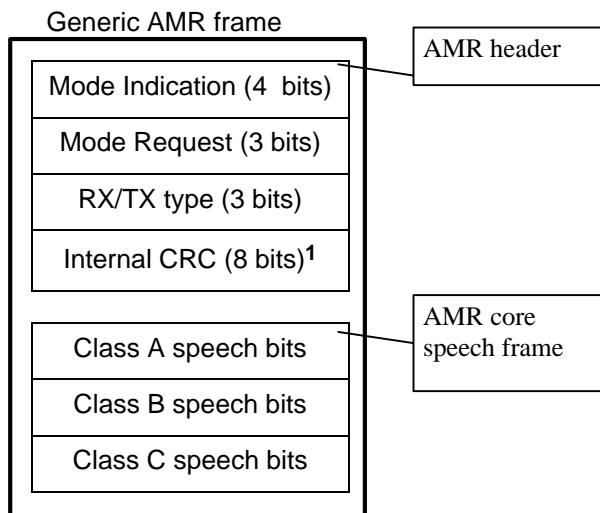
Figure 1. General frame structure
