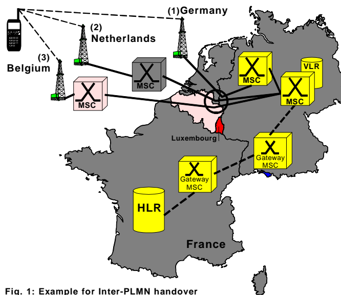
Fig. 1: Example for Inter-PLMN handover
