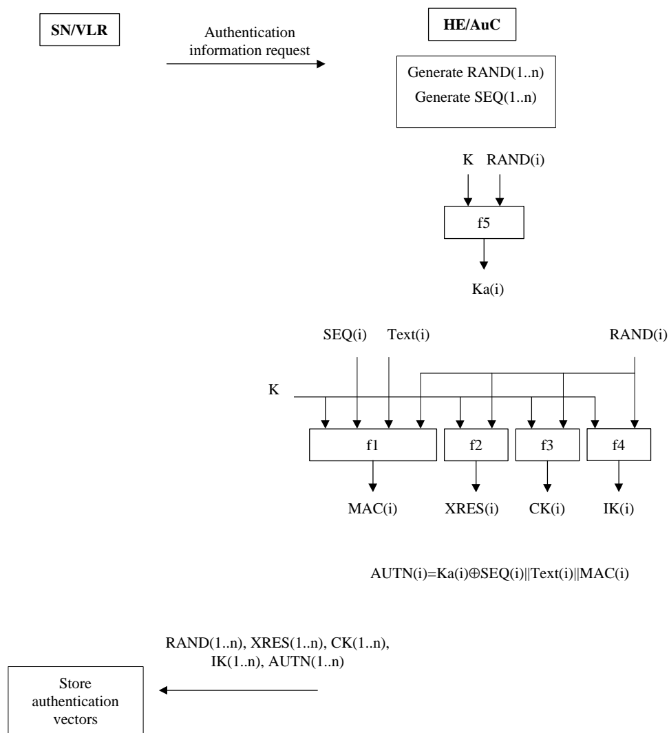
Figure Error! Style not defined..Error! Bookmark not defined. - Procedure for distributing authentication vectors from the HE/AuC to the SN/VLR
