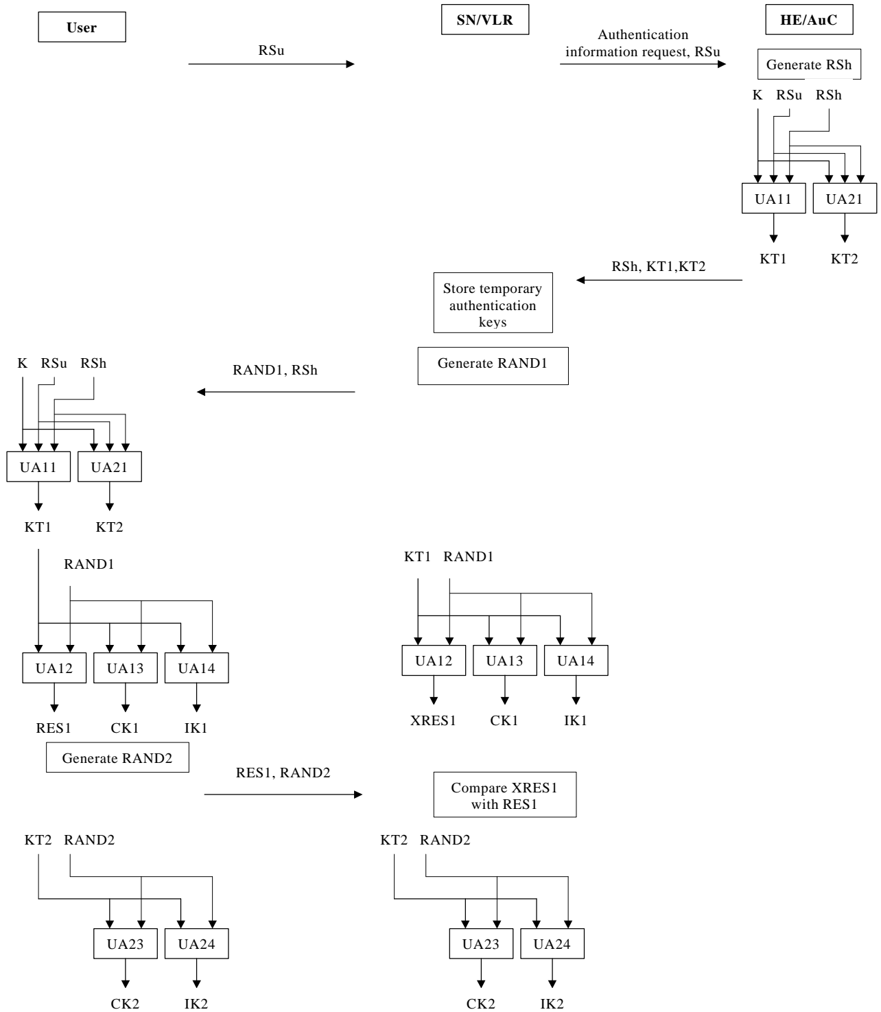
Figure Error! Style not defined..Error! Bookmark not defined. General procedure for new registrations
