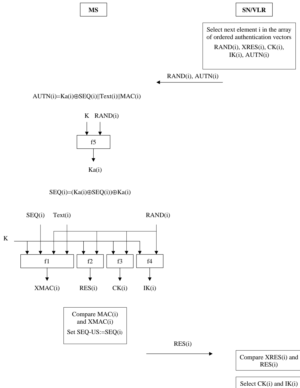
Figure Error! Style not defined..Error! Bookmark not defined. - Overview of authentication exchange
