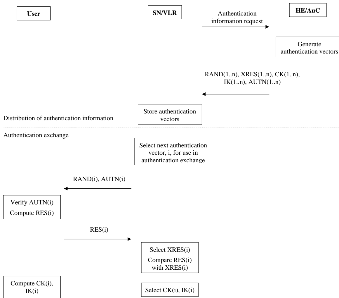
Figure Error! Style not defined..Error! Bookmark not defined. Overview of authentication and key establishment method
