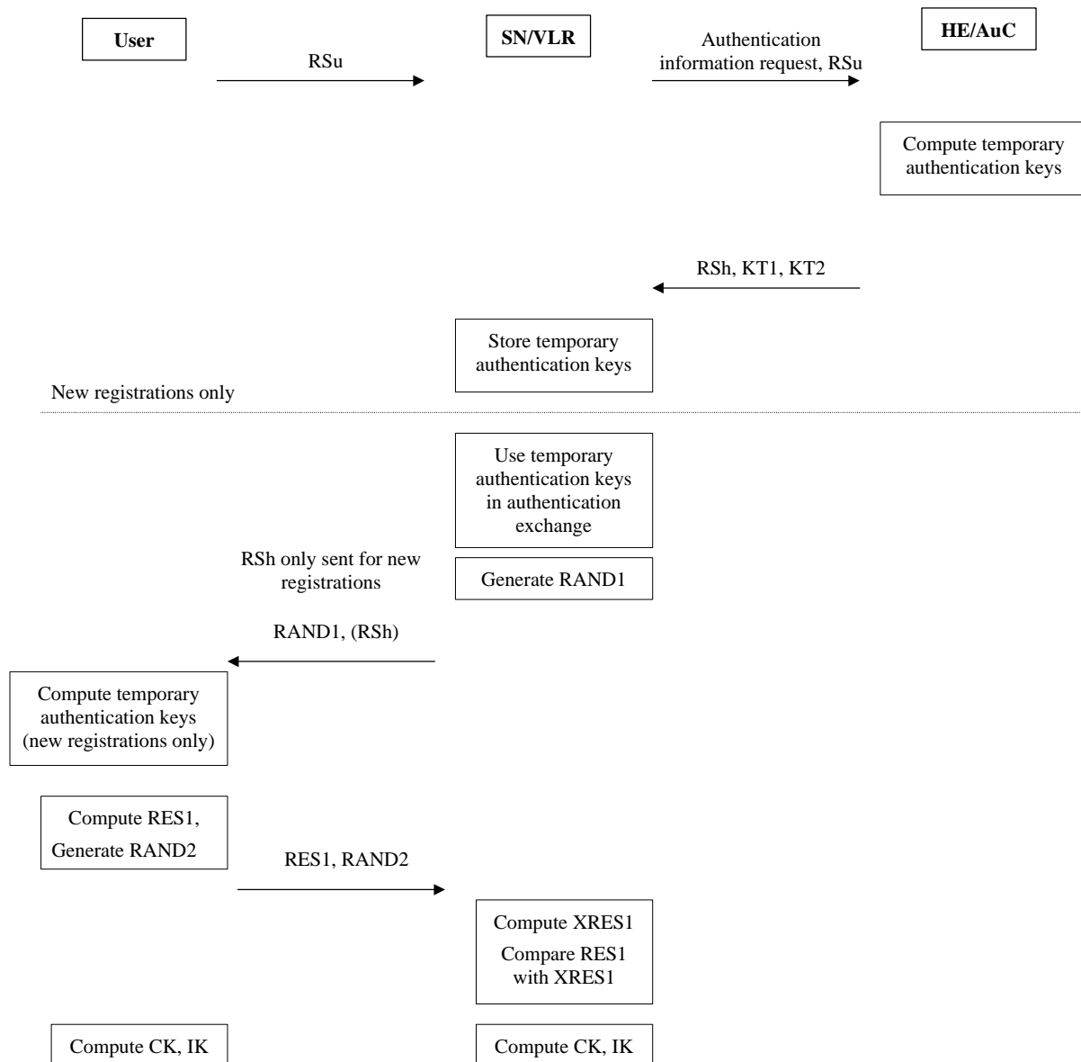
Figure Error! Style not defined..Error! Bookmark not defined. – Overview of authentication procedure
