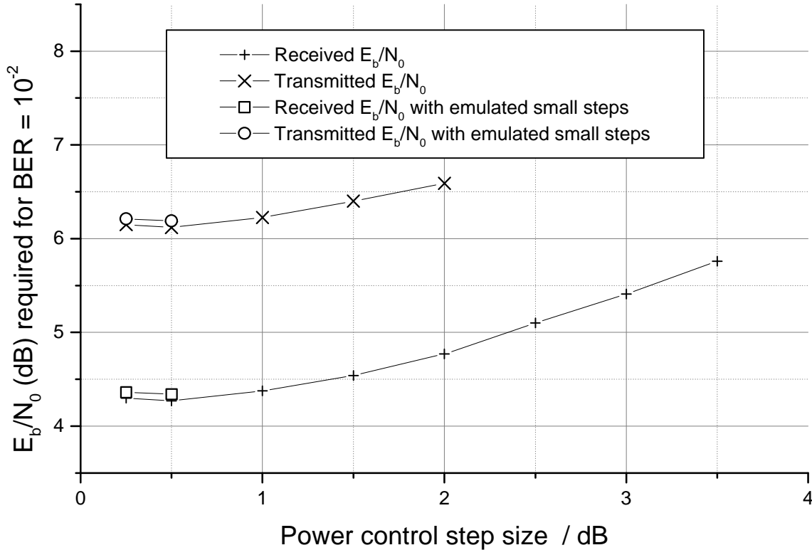
Figure 2 E_b/N_0 for BER=0.01, terminal speed 1km/hr, 6 path channel
