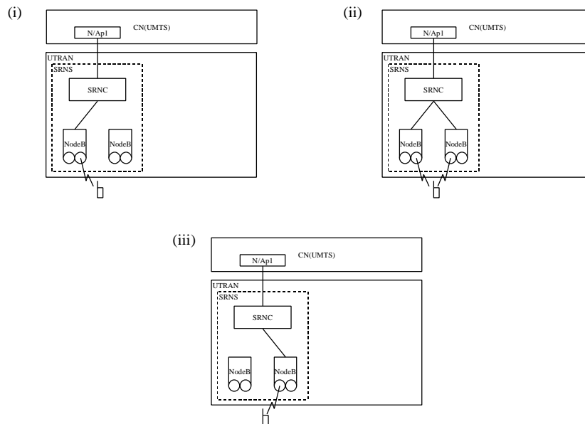
Inter Node B (Intra RNS)
