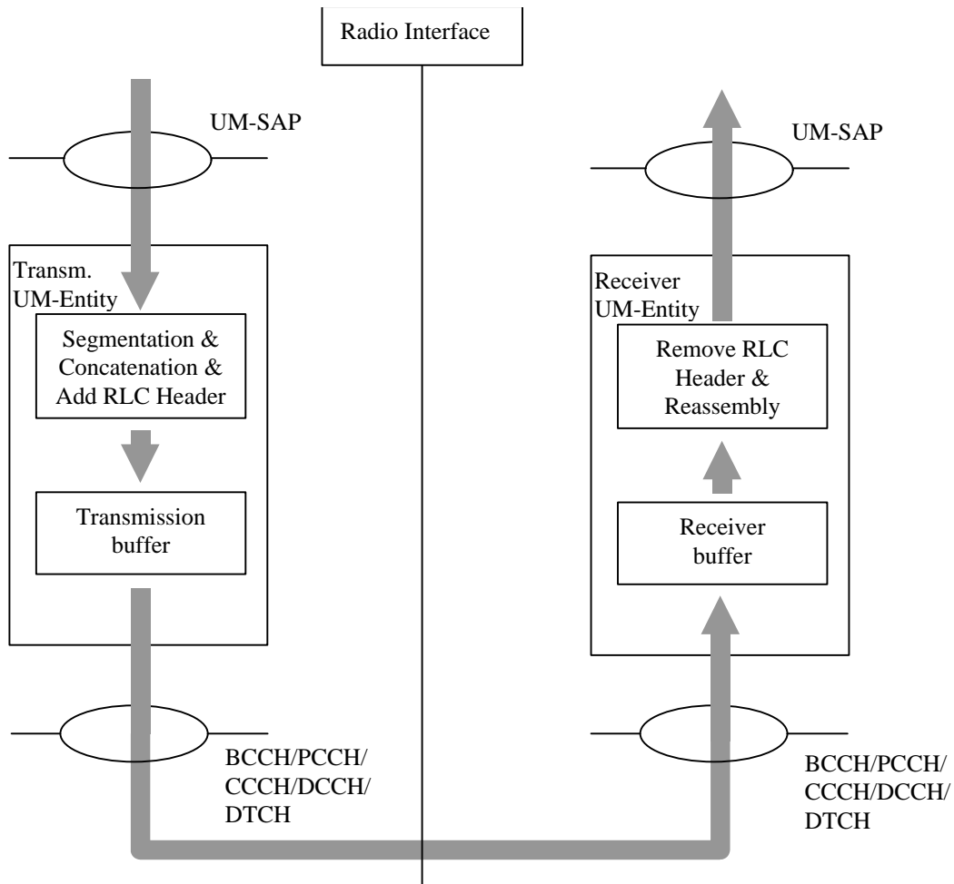
Figure Error! No text of specified style in document.-333 Model of two unacknowledged mode peer entities.
