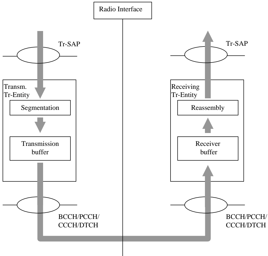
Figure Error! No text of specified style in document.-222 Model of two transparent mode peer entities.
