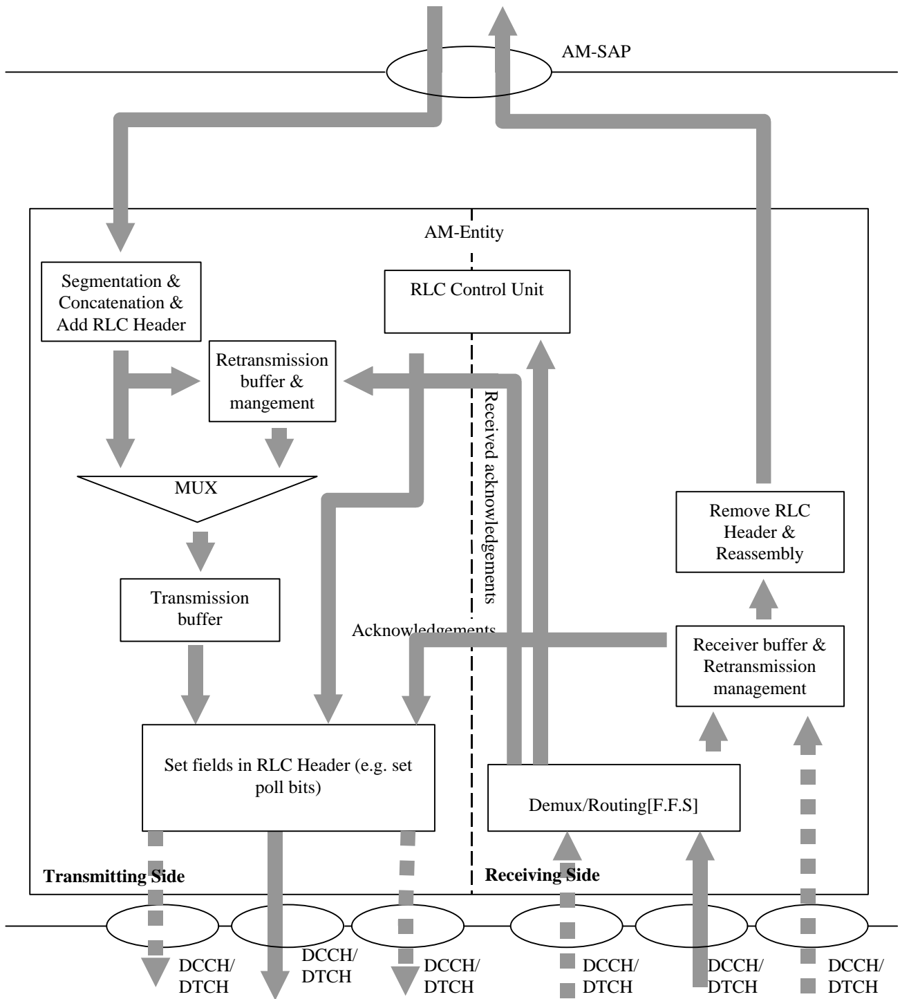
Figure Error! No text of specified style in document. -444 Model of a acknowledged mode entity.
