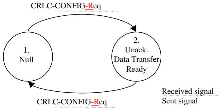
Figure Error! No text of specified style in document.-171717. The state model for unacknowledged mode entities.
