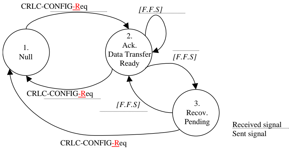
Figure Error! No text of specified style in document.-181818. The state model for the acknowledged mode entities.
