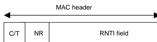
Figure 9.1.2.1 MAC control PDU ( ffs )
