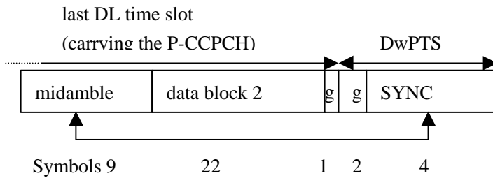
Figure: The frame structure around DwPTS
