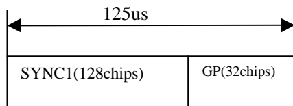
Figure Burst structure of UpPTS
