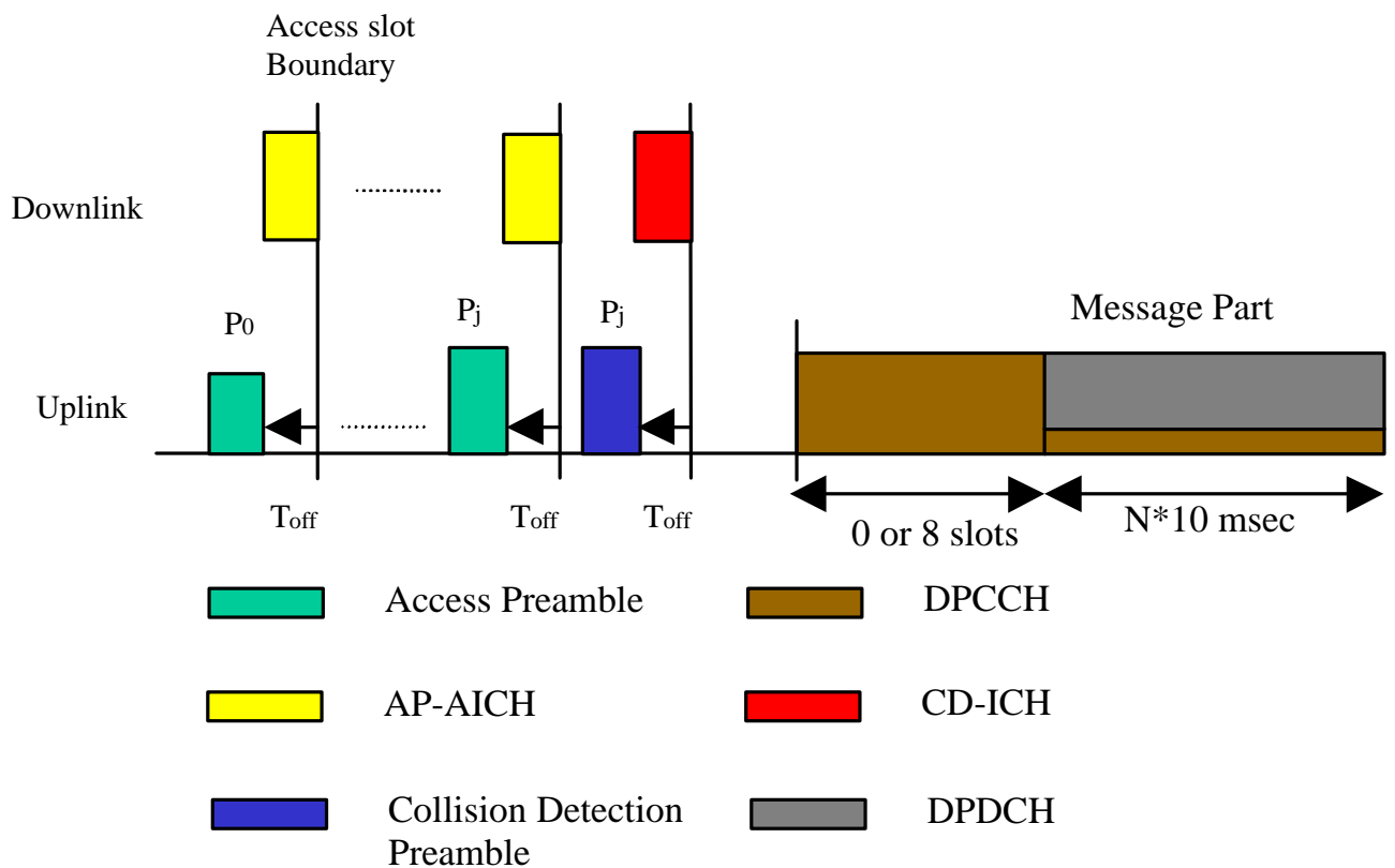
Figure 2: Structure of the CPCH random access transmission
