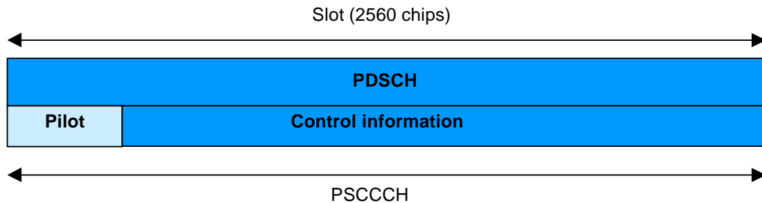
Figure 23: Frame structure for the DSCH when associated to a DSCH control channel.
