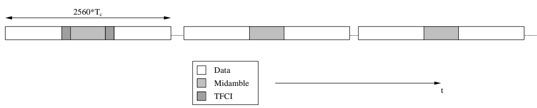
Figure 9: Example of TFCI transmission with physical channels multiplexed in time domain
