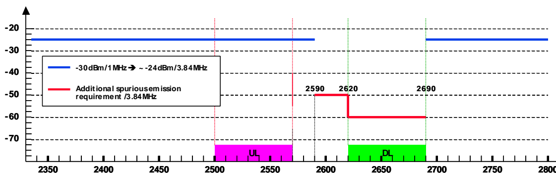
Figure XXX. Additional spurious emission requirement to protect the 2590-2620 MHz band
