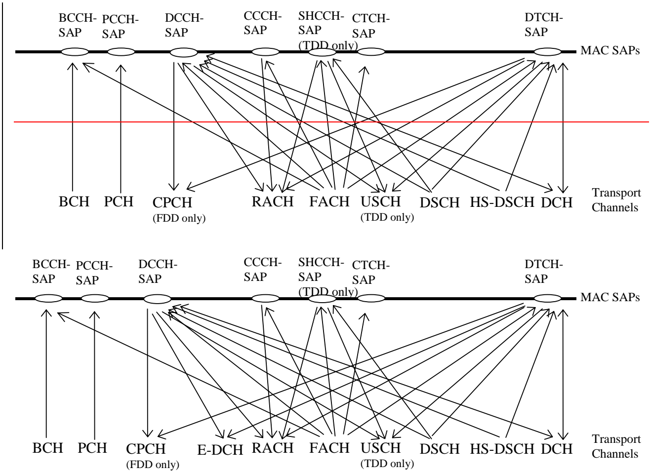
Figure 4: Logical channels mapped onto transport channels, seen from the UE side (Note to editor: Figure updated)
