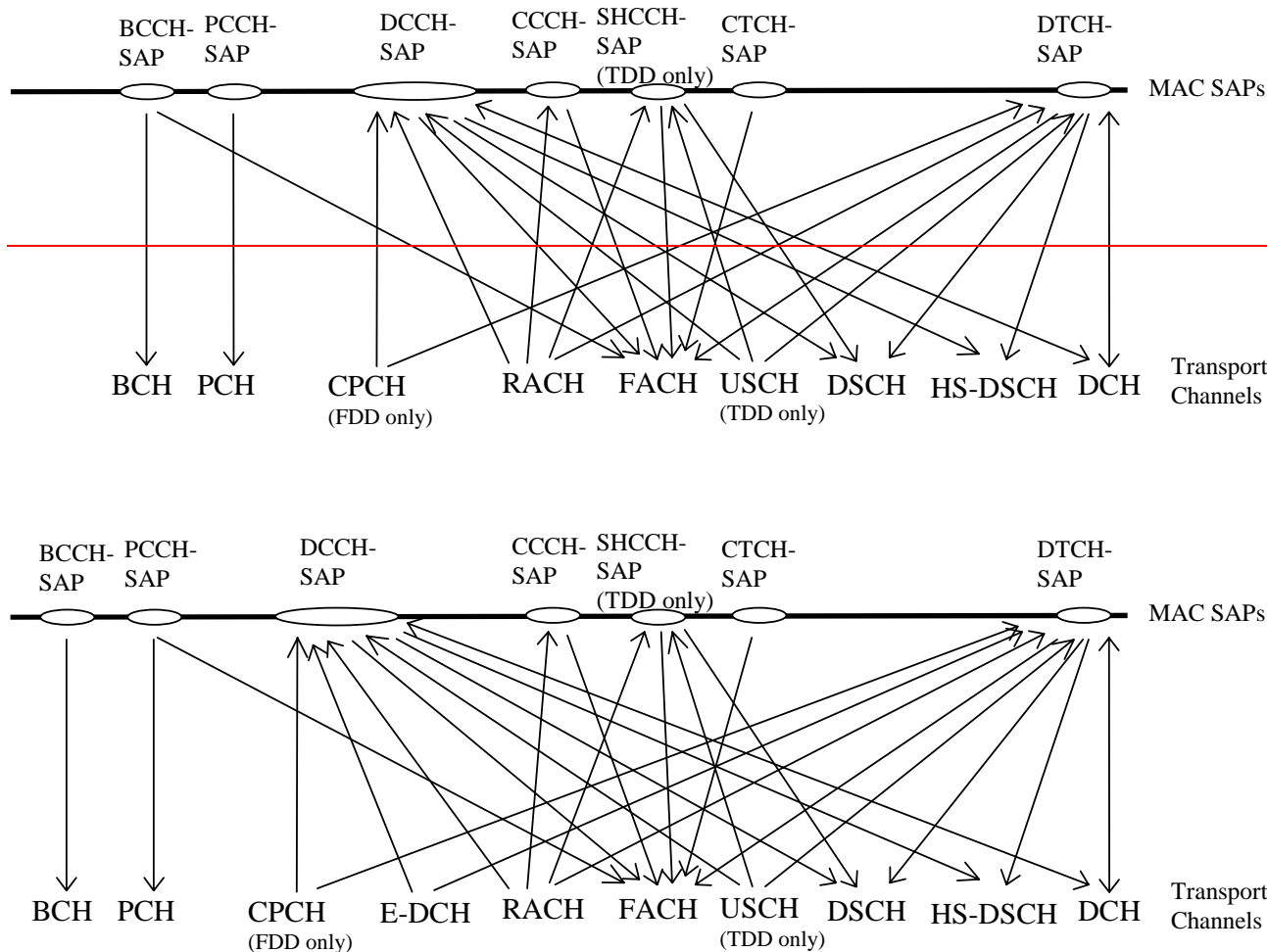
Figure 5: Logical channels mapped onto transport channels, seen from the UTRAN side (Note to editor: Figure updated)
