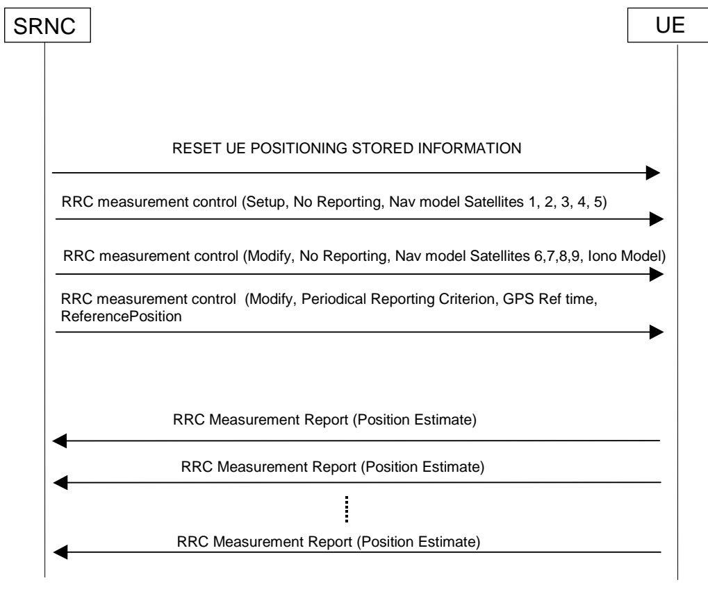
Figure D.2: UE-Based GPS Message Sequence Normal for moving scenario test case
