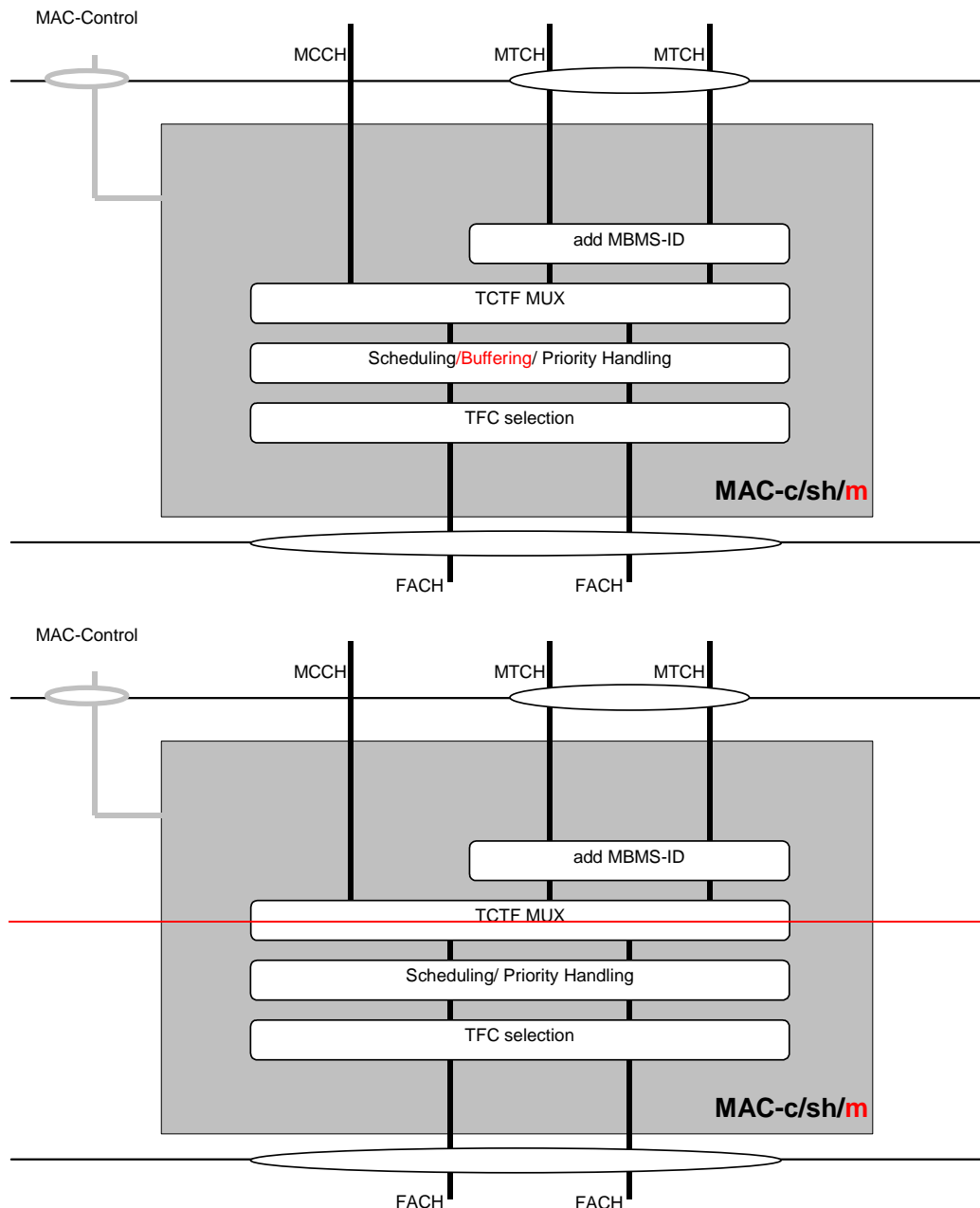
Figure 8: UTRAN side MAC-m architecture additions to MAC-c/sh
