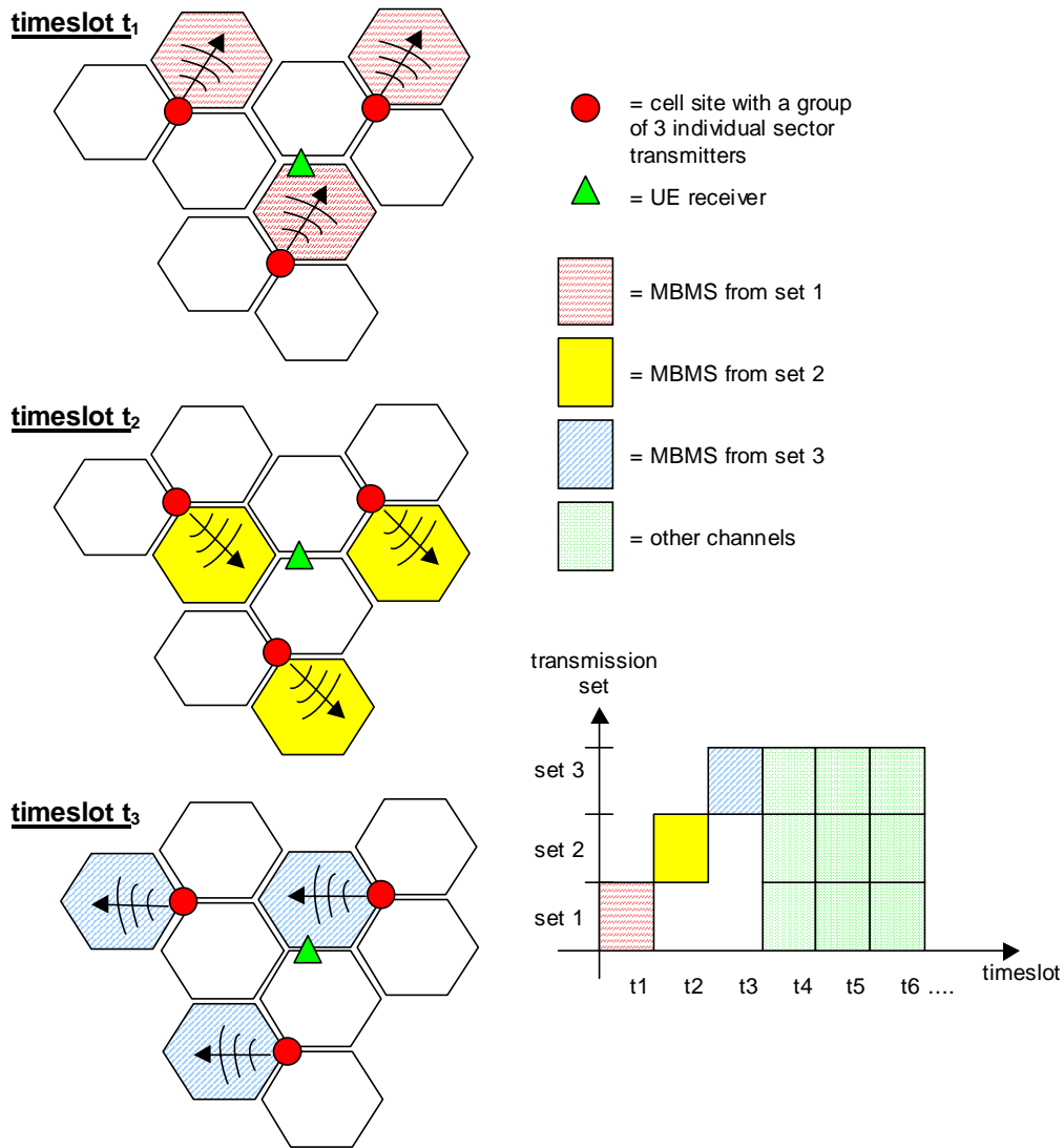
Figure 13: Example of non-time-coincident macro diversity transmission
