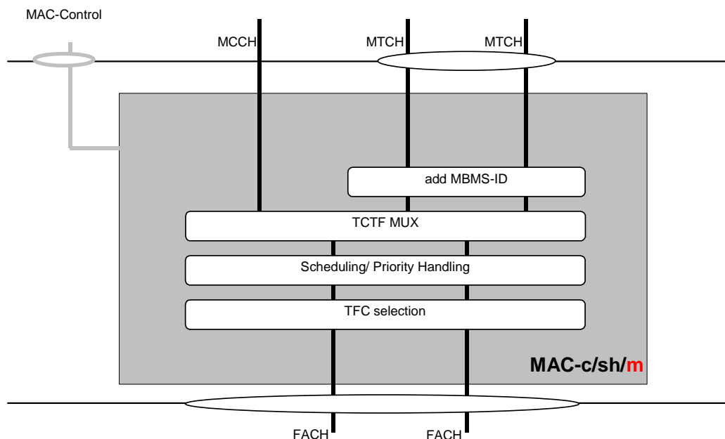
Figure 895: UTRAN side MAC-m architecture additions to MAC-c/sh
