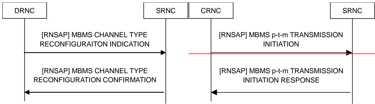
Figure 32322821 : Channel Type Reconfiguration MBMS p-t-m transmission initiation signalling flow: Successful Operation.
