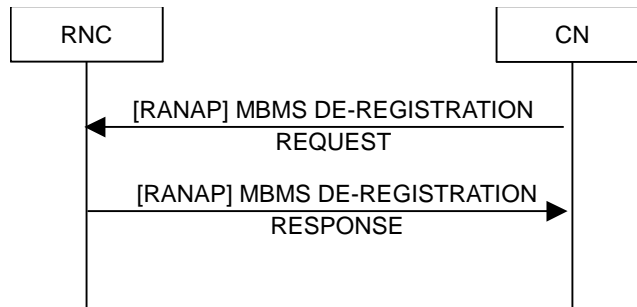
Figure 25252115 : CN MBMS De-Registration procedure.
