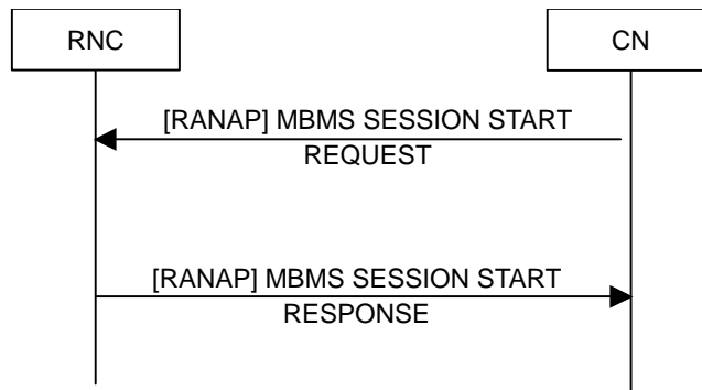
Figure 20201611: MBMS Session Start procedure. Successful operation.
