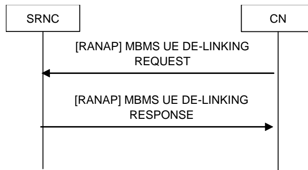
Figure 28282418 : MBMS UE De-linking signalling flow
