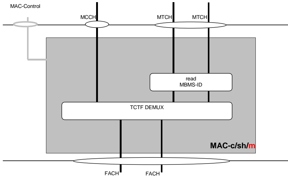
Figure 996: UE side MAC-m additions to MAC-c/sh
