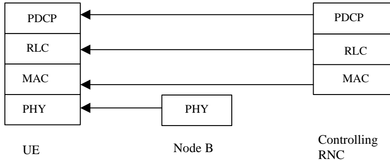
Figure 552: Protocol Stack for MTCH
