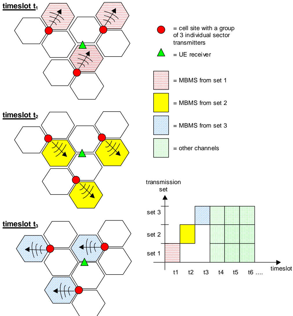
Figure 15: Example of non-time-coincident macro diversity transmission
