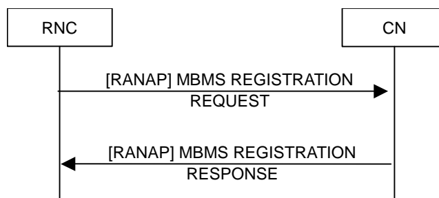
Figure 23231913 : MBMS Registration procedure.
