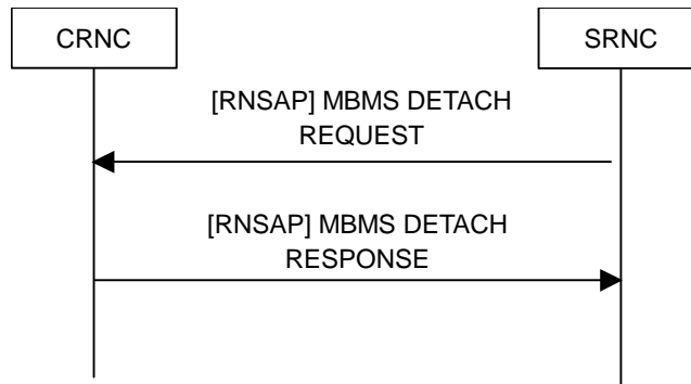
Figure 31312720 : MBMS detach request signalling flow: Successful Operation.
