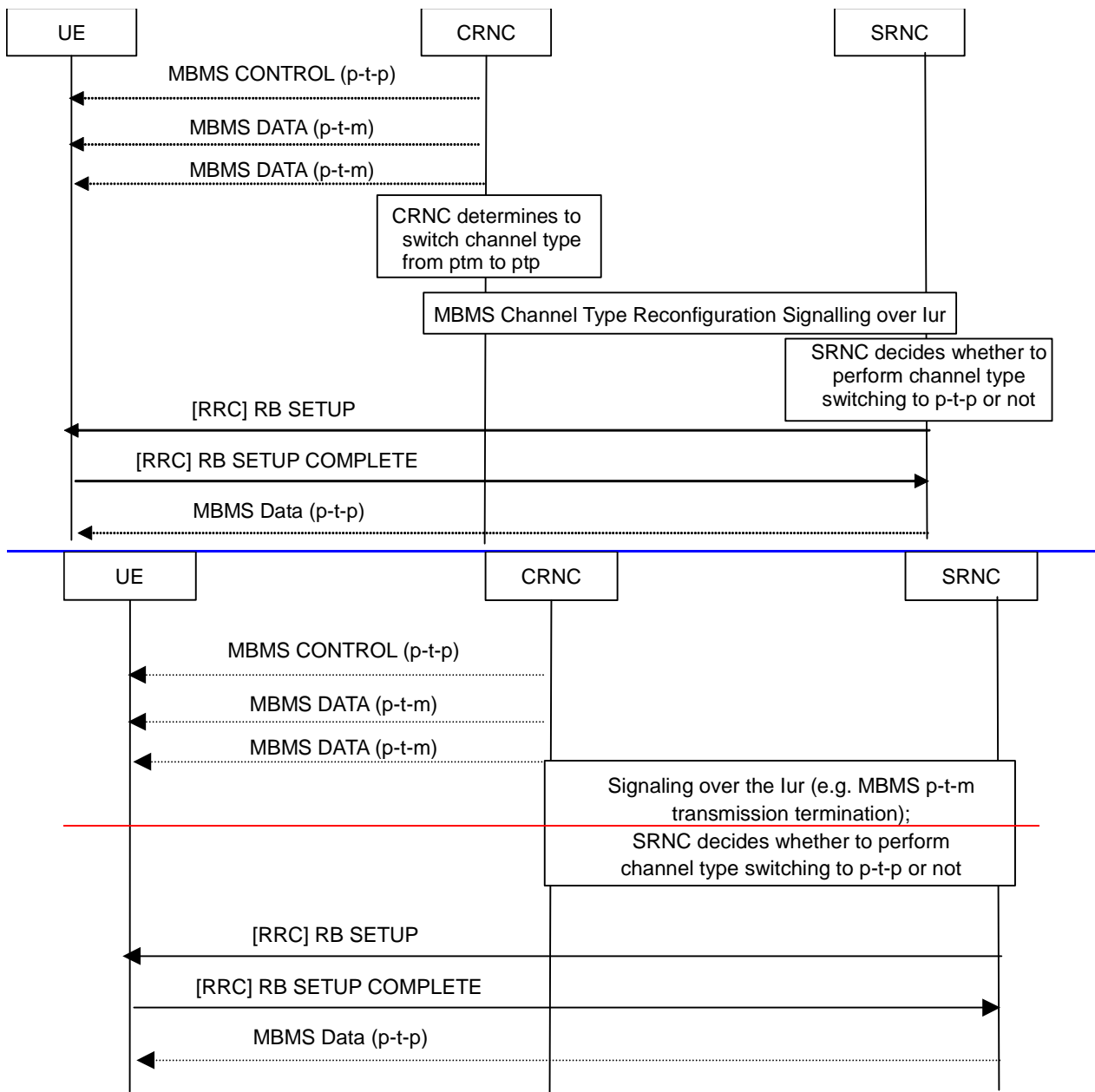
Figure 26262216 : Channel type switching signalling flow from p-t-m to p-t-p.
