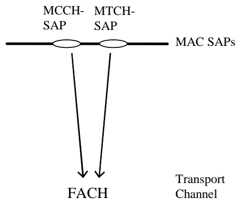
Figure 13 Figure 13 Figure 10 : Logical channels mapped onto transport channel, seen from the UTRAN side
