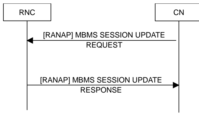
Figure 212117: MBMS Session Update procedure. Successful operation.
