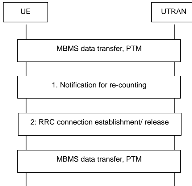
Figure 18: Figure 3 -Recounting with continuation of p-t-m PTM
