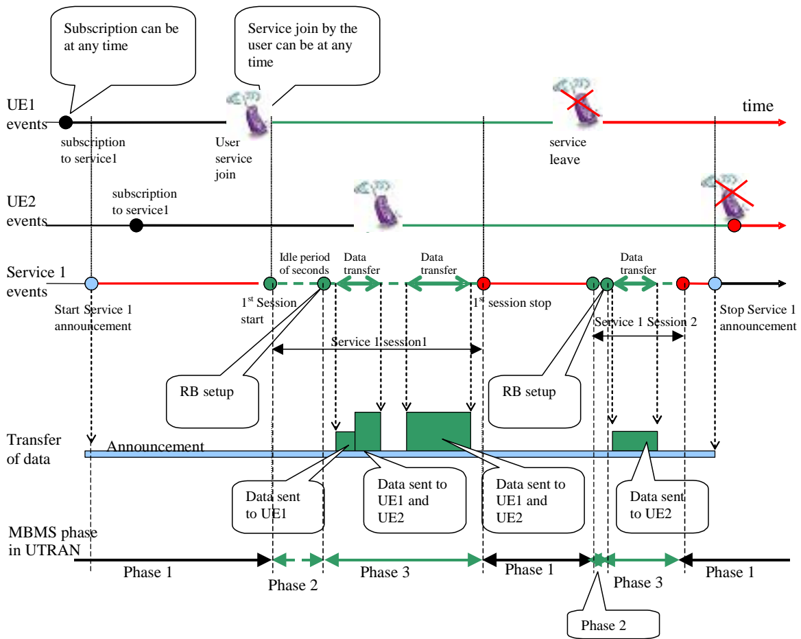
Figure 43433929: Timeline of MBMS Service
