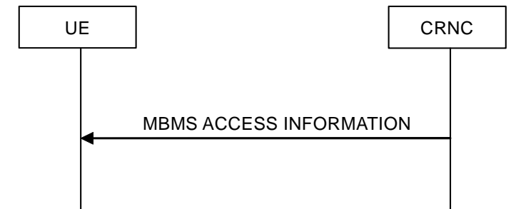
Figure 37333: MBMS Access Information signalling flow
