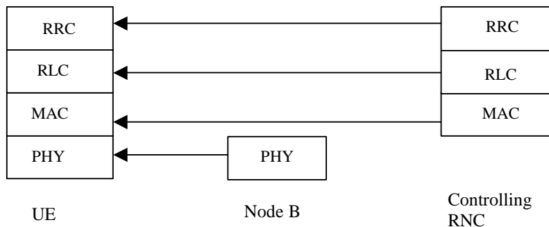
Figure 663: Protocol Stack for MCCH
