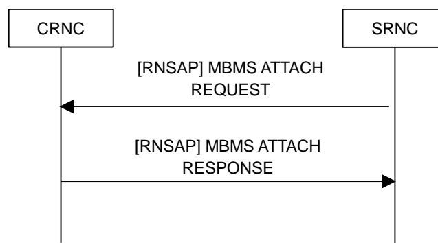
Figure 302619: MBMS attach request signalling flow: Successful Operation.
