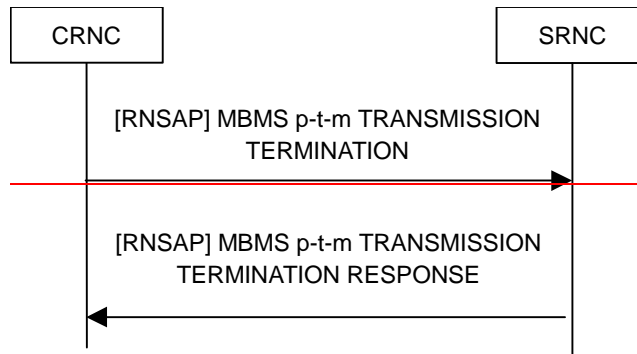
Figure 22- MBMS p-t-m transmission termination signalling flow: Successful Operation.
