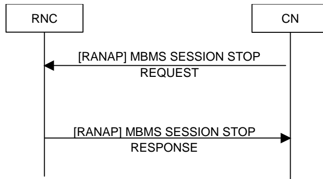
Figure 22221812 : MBMS Session Stop procedure.
