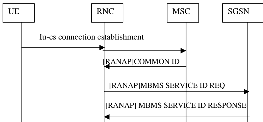
Figure 27: MBMS Service Id list over lu signalling flow
