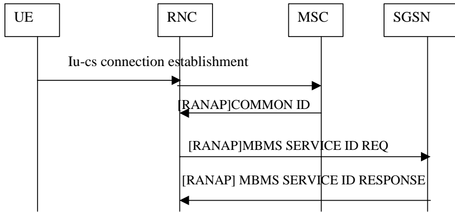
Figure 2925: MBMS Service Id list over Iu signalling flow
