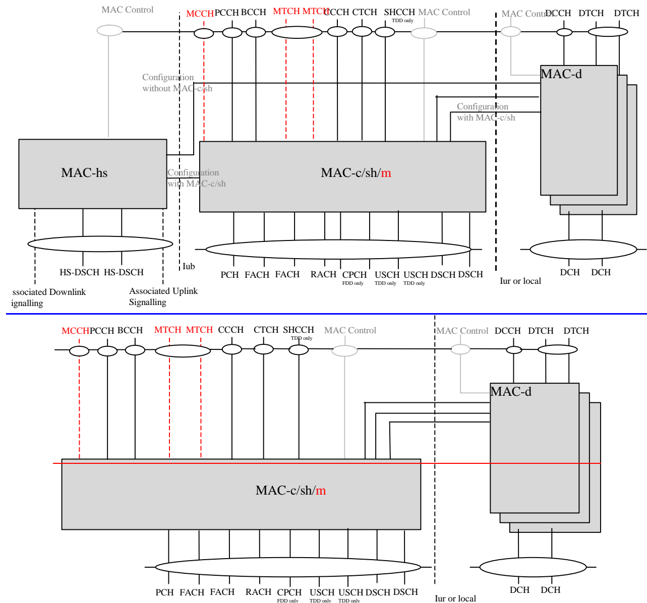
Figure 7.4: UTRAN MAC architecture
