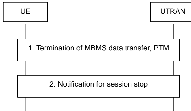
Figure 19 Figure 4 : Session stop
