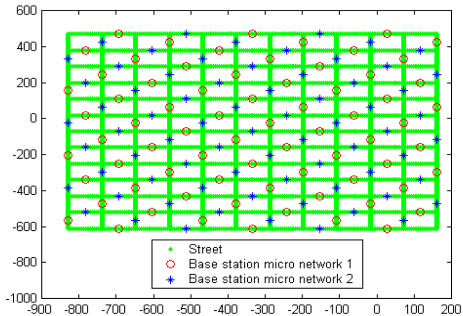
FigureA.7: Micro-Micro layout [units in meter].
