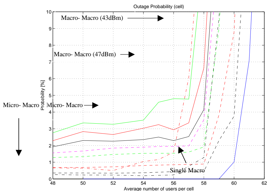
Figure A.20: Outage probability for the users connected to the macro cells for macro site-to-site distance of 1 km and a fixed maximum output power of up to 37dBm per Medium Range BS
