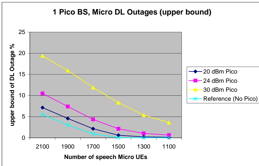
Figure A.24 Upper bound of micro layer DL Outage due to 1 LA BS with 20, 24, 30 dBm TX power
