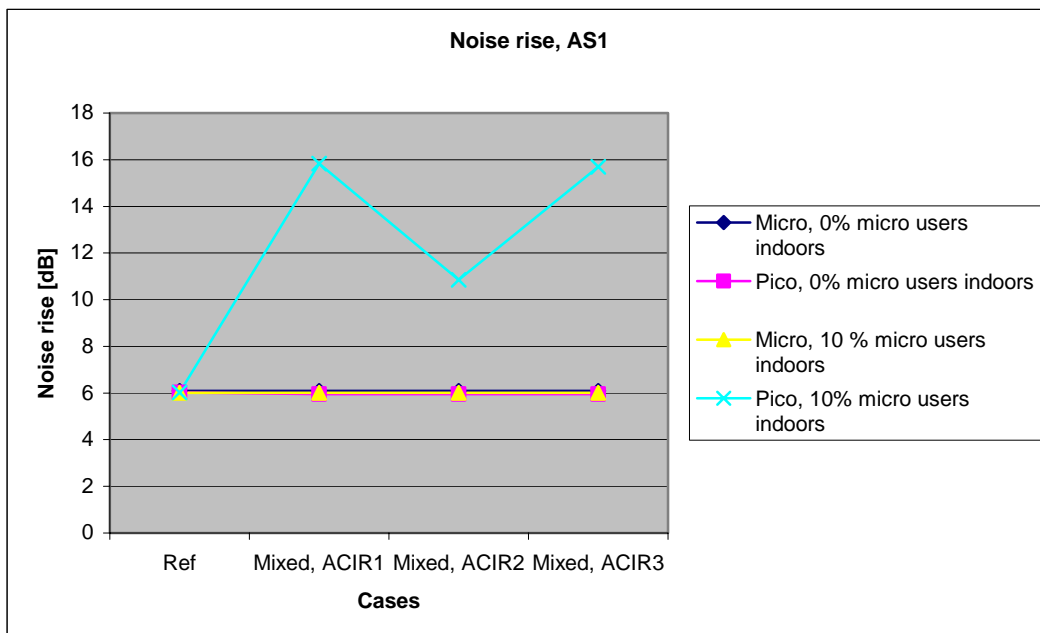
Figure A.13: UL noise rise versus ACIR value
