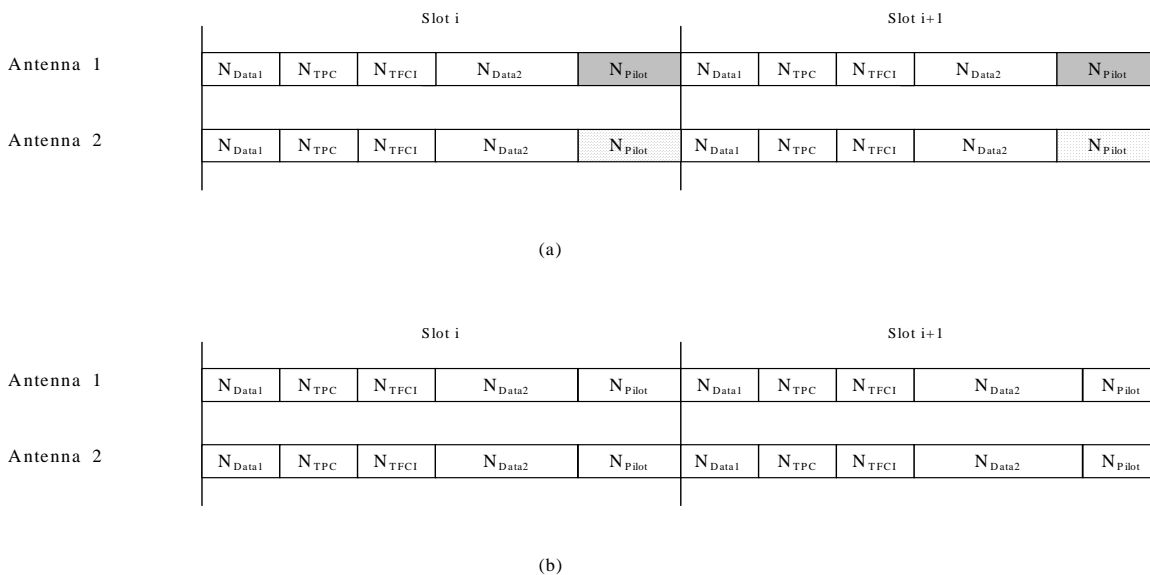
Figure 113: Slot structures for downlink dedicated physical channel diversity transmission. Structure (a) is used in closed loop mode 1. Structure (b) is used in closed loop mode 2. Different shading of the pilots indicate orthogonality of the patterns
