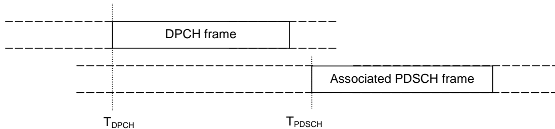
Figure 337: Timing relation between DPCH frame and associated PDSCH frame
