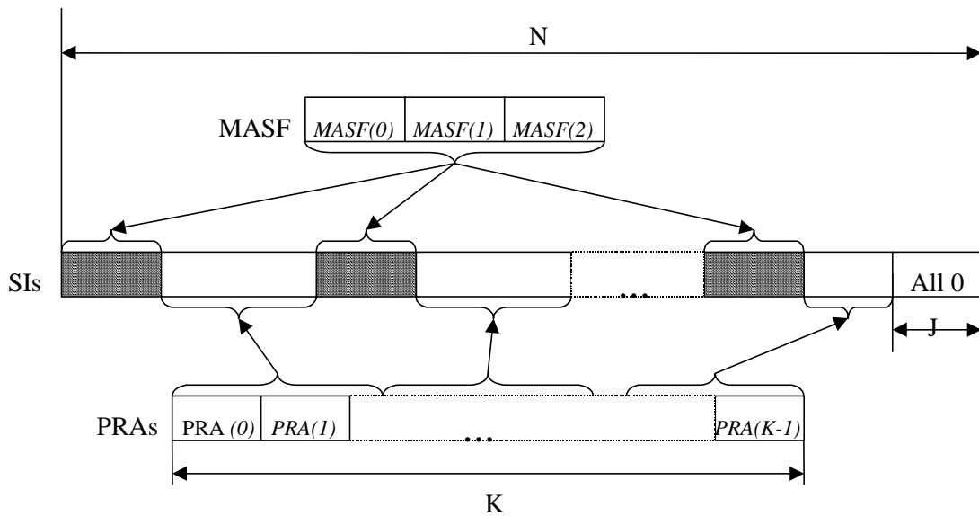
Figure 268: Mapping of MASF and PRAs to SIs in CSICH
