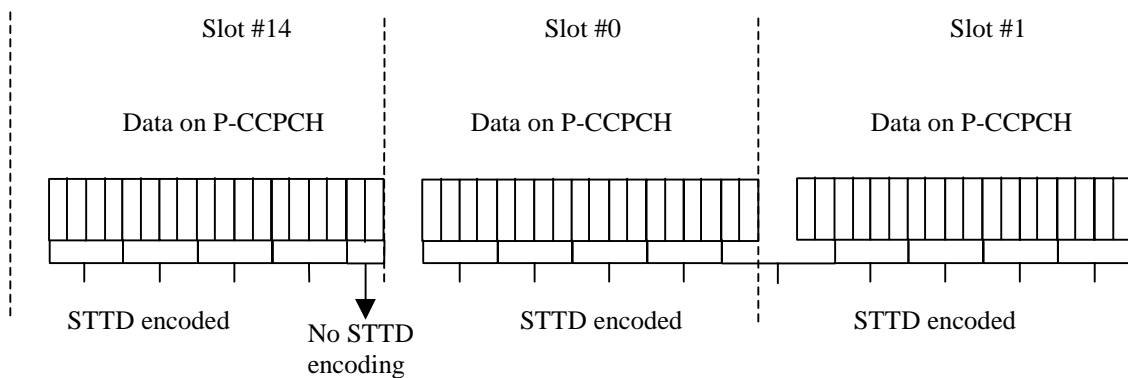
Figure 168: STTD encoding for the data bits of the P-CCPCH
