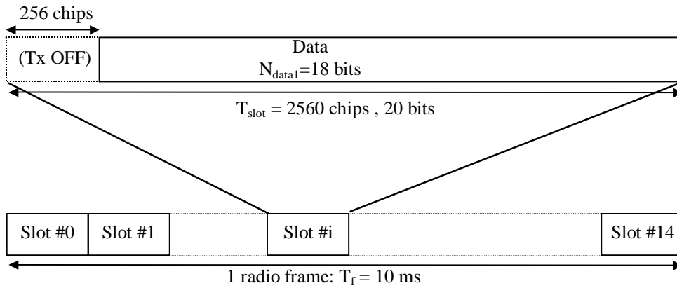
Figure 157: Frame structure for Primary Common Control Physical Channel
