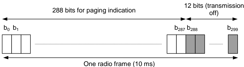
Figure 246: Structure of Paging Indicator Channel (PICH)
