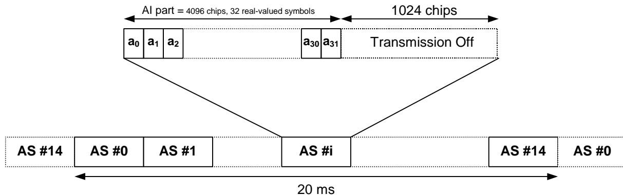
Figure 213: Structure of Acquisition Indicator Channel (AICH)
