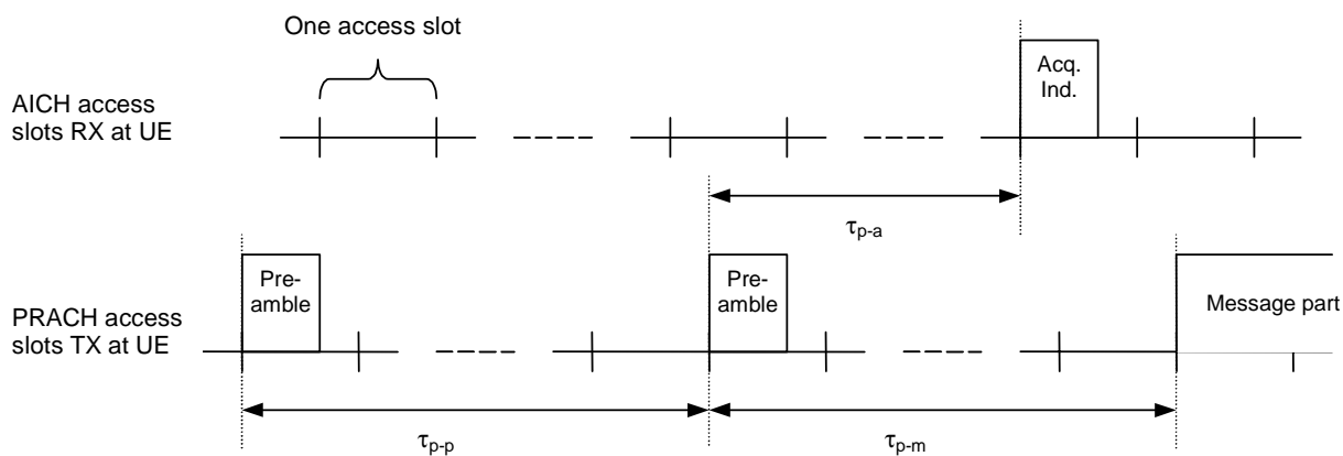
Figure 315: Timing relation between PRACH and AICH as seen at the UE
