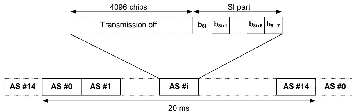
Figure 257: Structure of CPCH Status Indicator Channel (CSICH)
