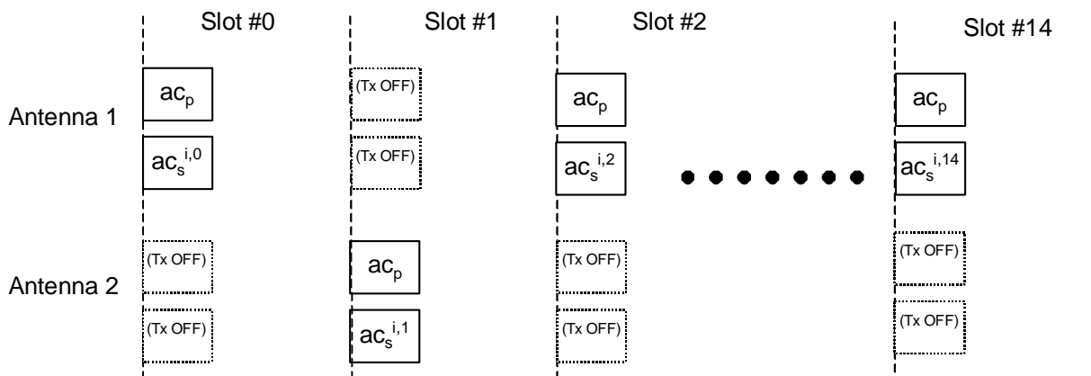
Figure 1924: Structure of SCH transmitted by TSTD scheme
