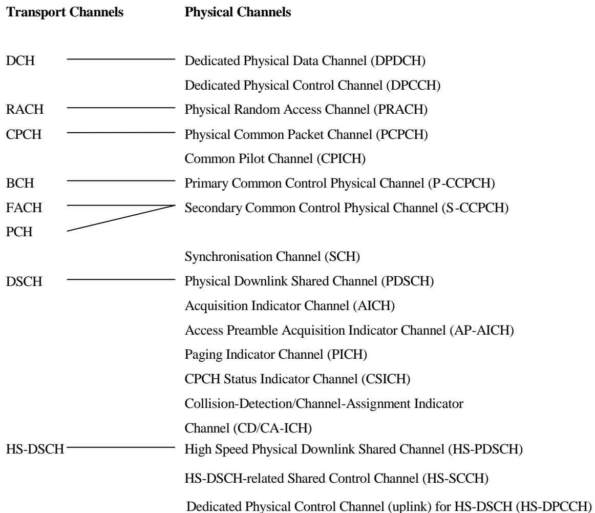
Figure 31: Transport-channel to physical-channel mapping
