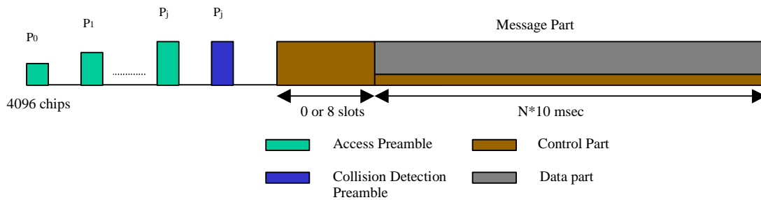
Figure 76: Structure of the CPCH access transmission
