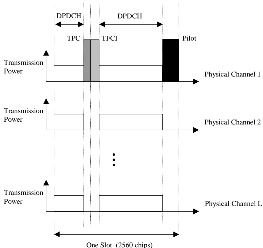
Figure 102: Downlink slot format in case of multi-code transmission
