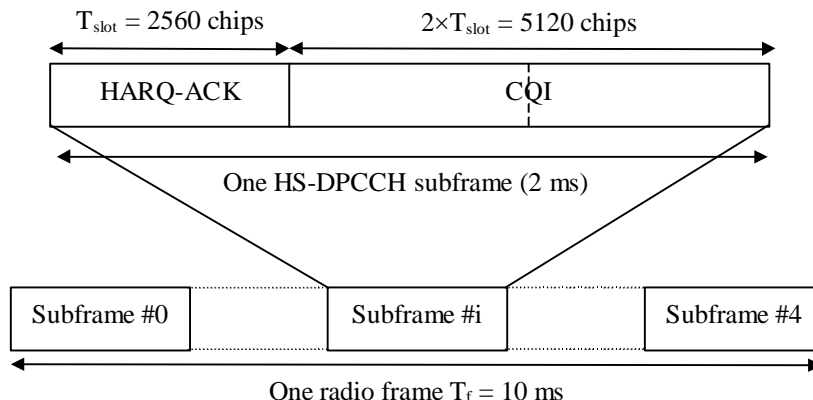
Figure 32A: Frame structure for uplink HS-DPCCH
