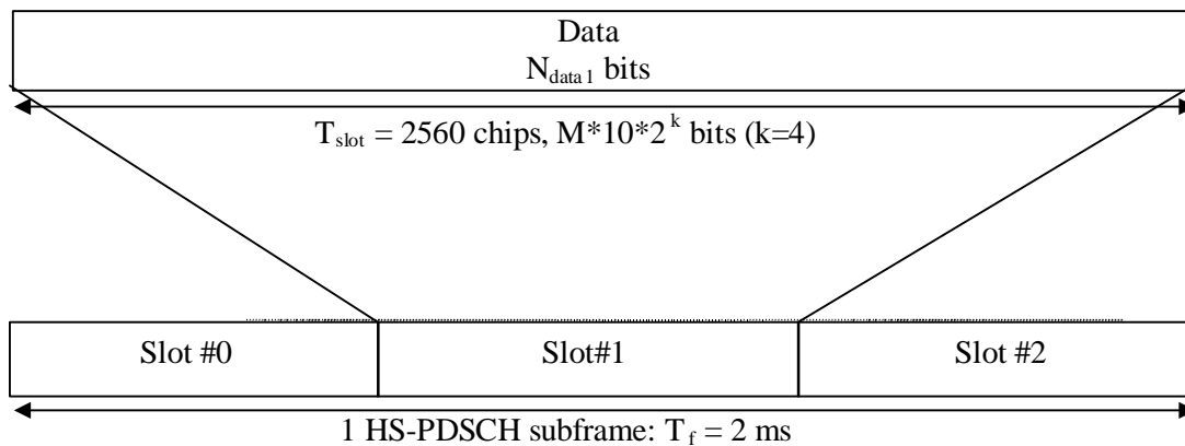
Figure 26B30: Subframe structure for the HS-PDSCH
