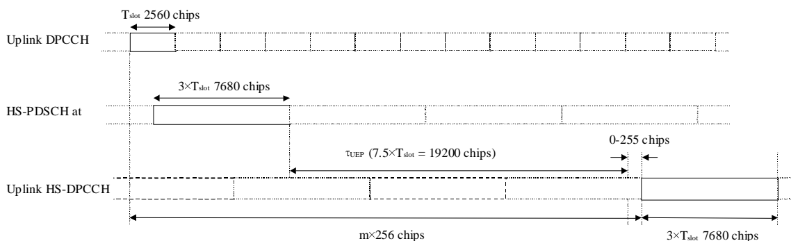
Figure 348: Timing structure at UE for HS-DPCCH control signalling
