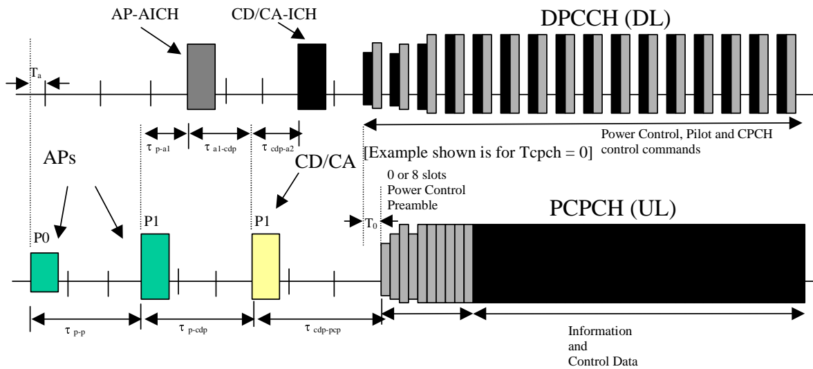
Figure 362: Timing of PCPCH and AICH transmission as seen by the UE, with T_{cpch} = 0
