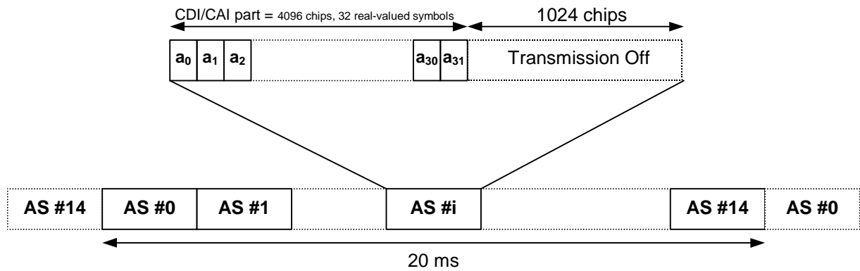
Figure 235: Structure of CD/CA Indicator Channel (CD/CA-ICH)
