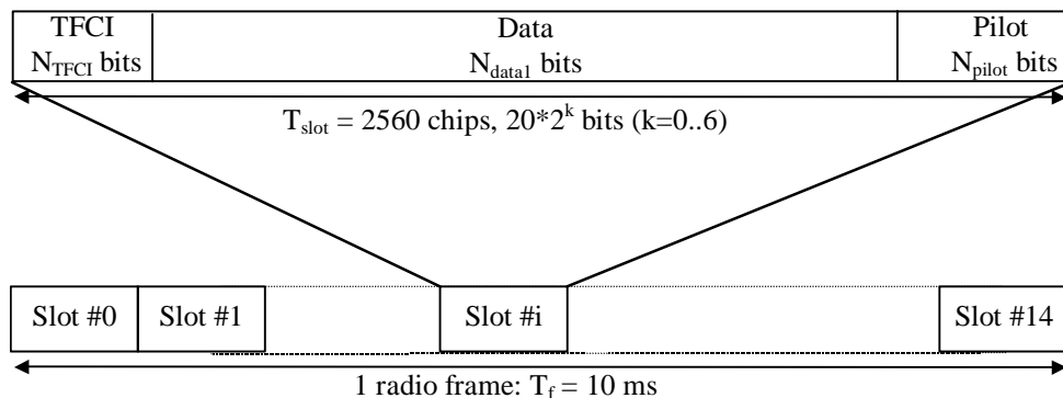
Figure 179: Frame structure for Secondary Common Control Physical Channel
