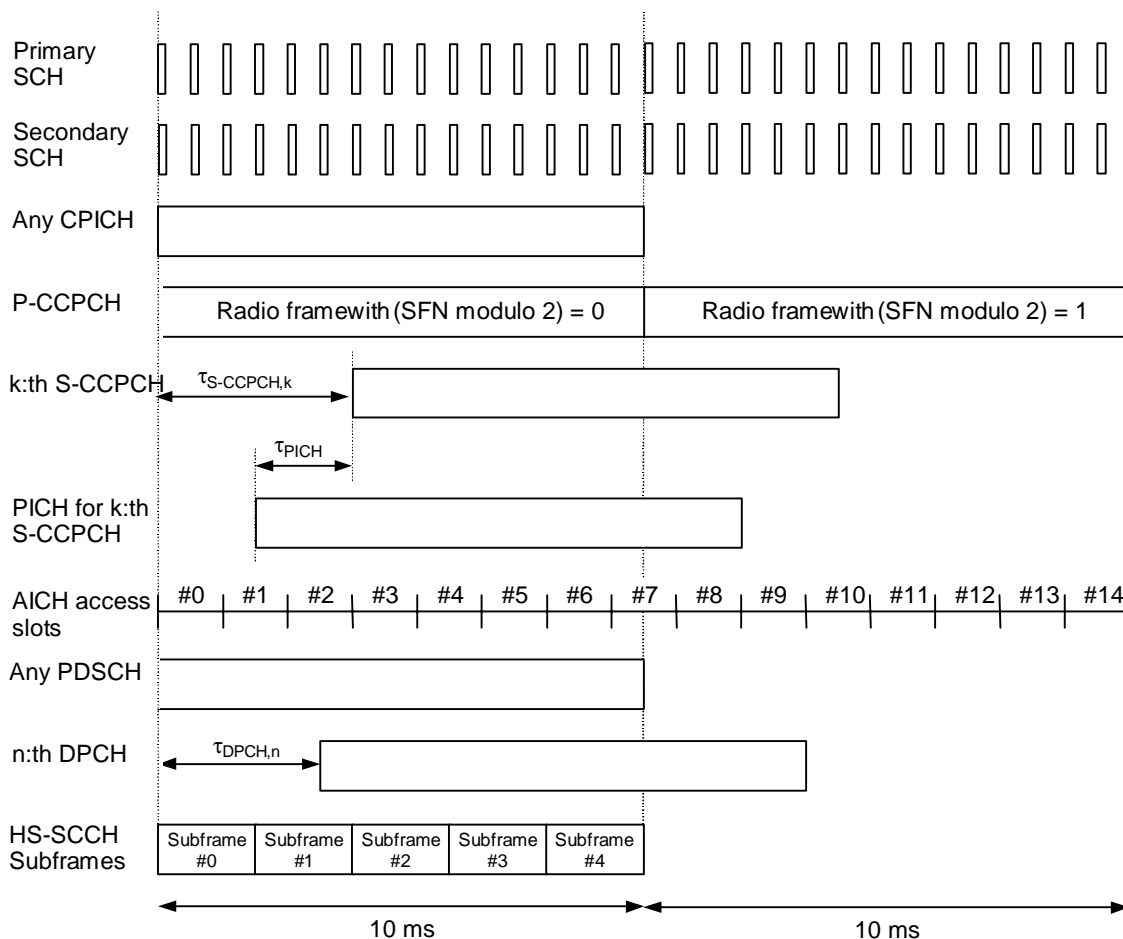
Figure 2933: Radio frame timing and access slot timing of downlink physical channels
