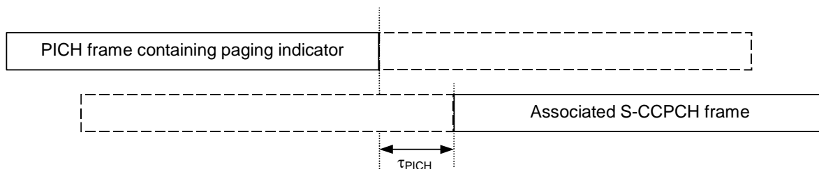
Figure 304: Timing relation between PICH frame and associated S-CCPCH frame
