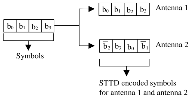
Figure 98: Generic block diagram of the STTD encoder for QPSK
