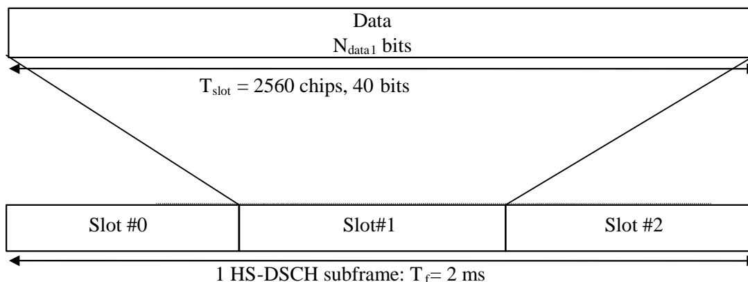
Figure 26A9: Subframe structure for the HS-SCCH
