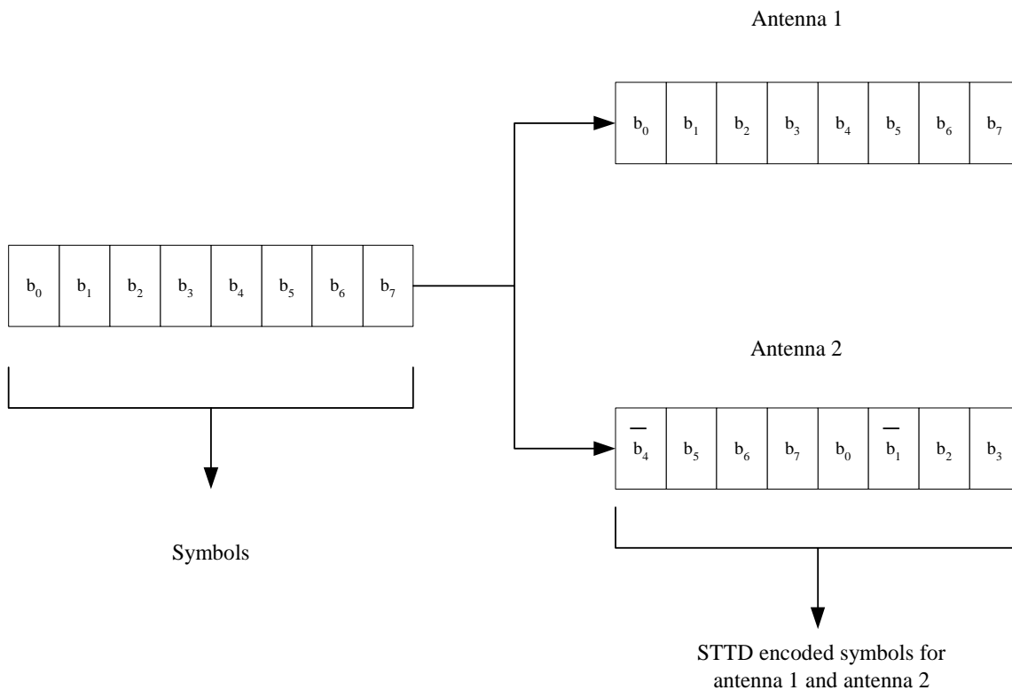
Figure 108A: Generic block diagram of the STTD encoder for 16QAM
