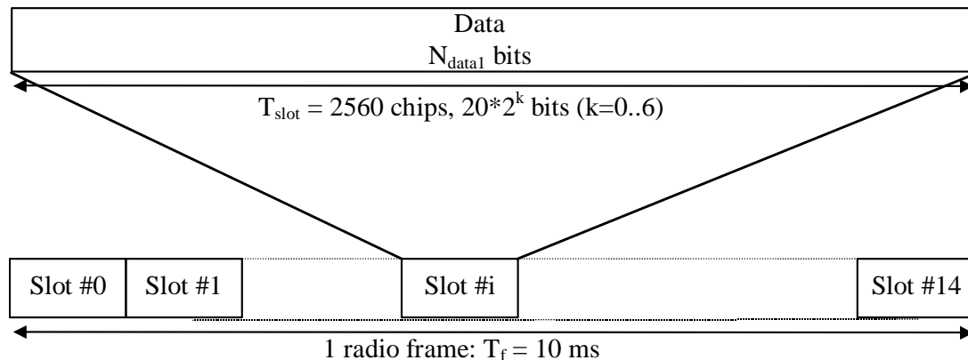
Figure 202: Frame structure for the PDSCH
