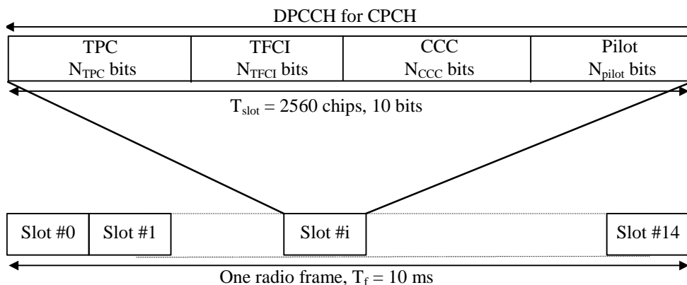
Figure 124: Frame structure for downlink DPCCH for CPCH
