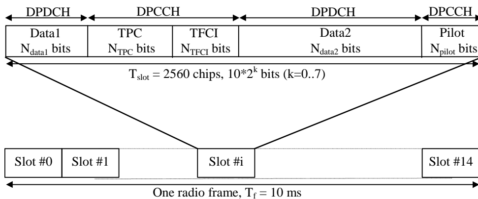
Figure 419: Frame structure for downlink DPCH
