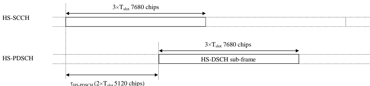
Figure 359: Timing relation between the HS-SCCH and the associated HS-PDSCH.
