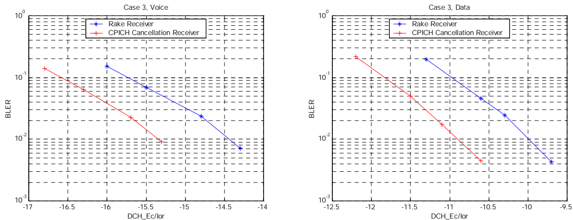
Figure 16: Block error rate as a function of DCH_Ec/Ior for RAKE and Pilot Mitigation receivers, (using the ideal assumptions of Annex B). Results are shown for Case 3 12.2 kbps and 64kbps channels.
