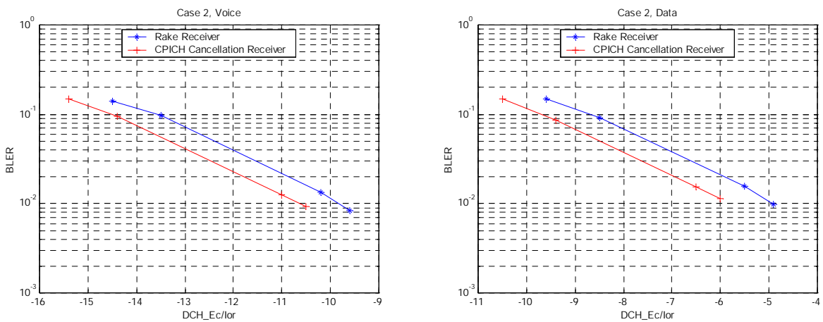
Figure 15: Block error rate as a function of DCH_Ec/Ior for RAKE and Pilot Mitigation receivers, (using the ideal assumptions of Annex B). Results are shown for Case 2 12.2 kbps and 64kbps channels.
