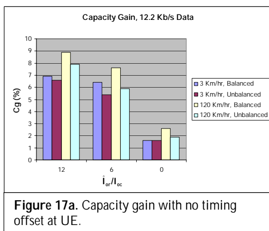
Figure 17: Capacity gain with and without timing offset at UE.
